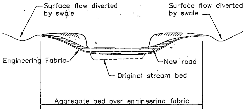
TYPICAL FORD CROSSING NOT TO SCALE
