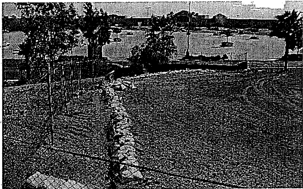
Gravel bags used as perimeter control.
