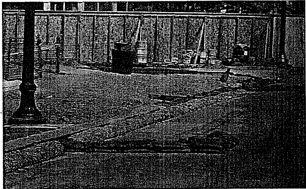
Gravel bags and fiber rolls used as a perimeter sediment control system.
