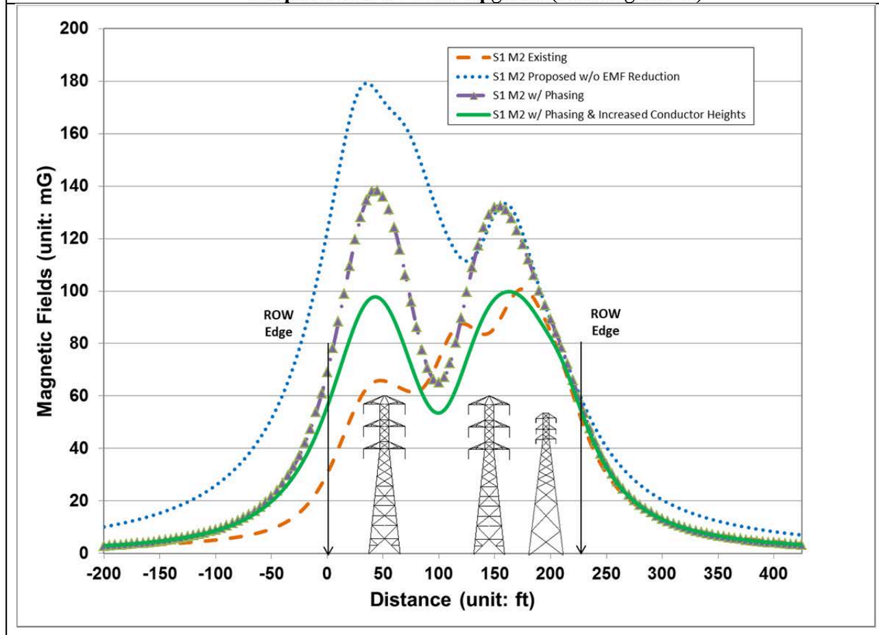
Figure 6. Calculated Magnetic Field Levels 49 for Segment 1 Model 2 Proposed 220 kV Line Upgrade (Looking North)
