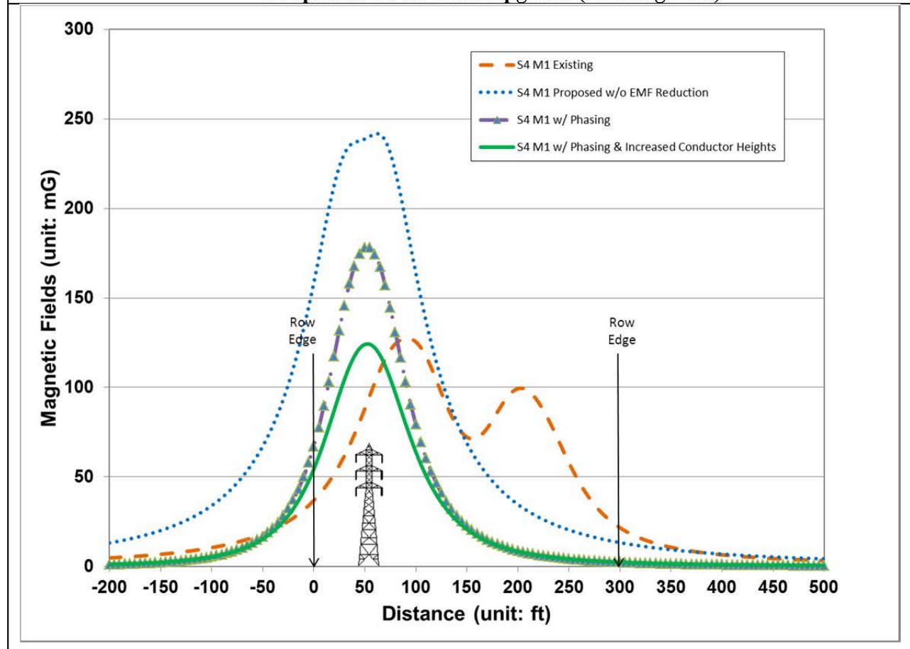
Figure 18. Calculated Magnetic Field Levels 73 for Segment 4 Model 1 Proposed 220 kV Line Upgrade (Looking East)
