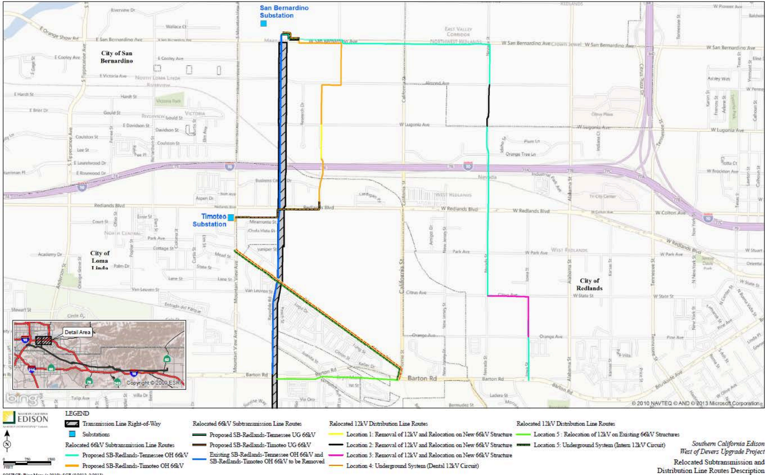
Figure 2. West of Devers Upgrade Project Subtransmission Relocation
