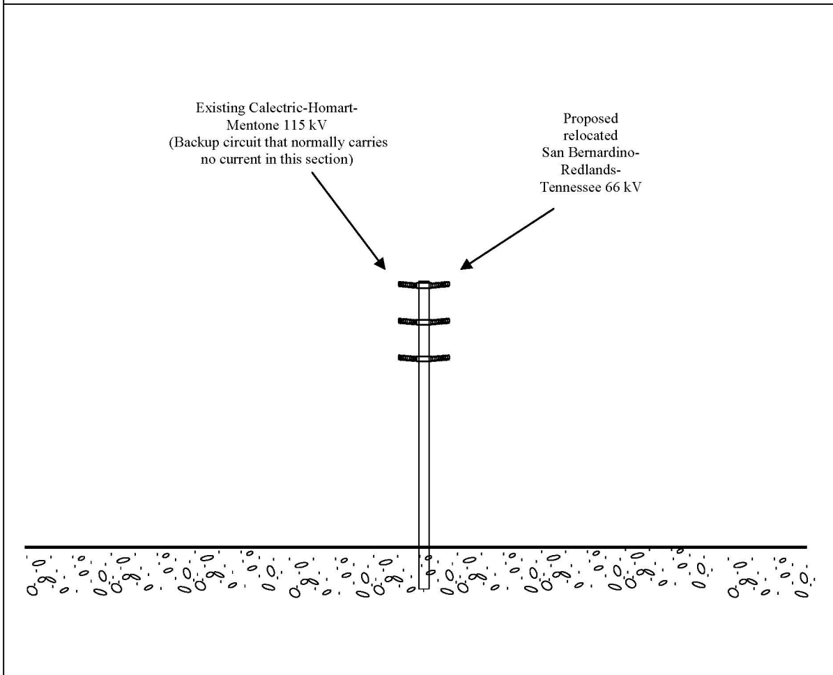
Figure 42. Proposed 66 kV Structures Design – San Bernardino-Redlands-Tennessee 66 kV Relocation Model 2 (on San Bernardino Avenue Looking East) 119
