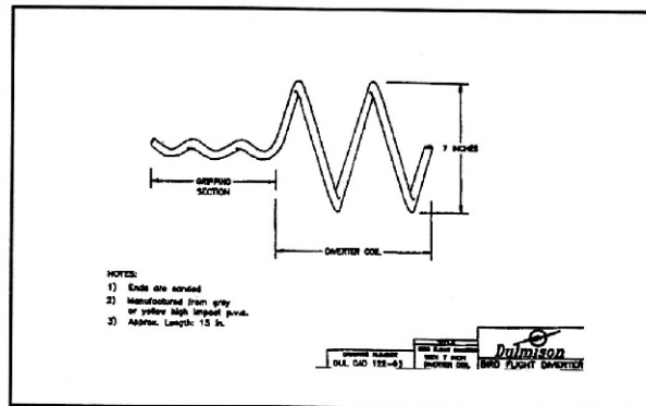
Figure 17 Bird flight diverter (BFD-7)
