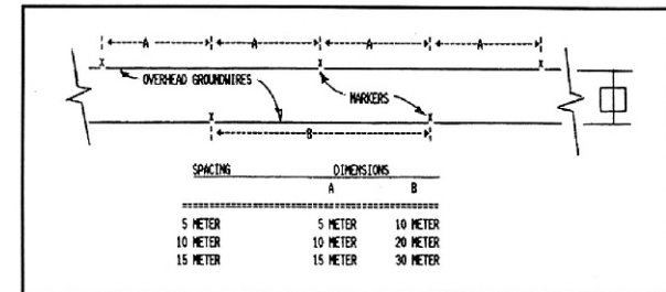
Figure 18 Marker spacing diagram for overhead groundwires
