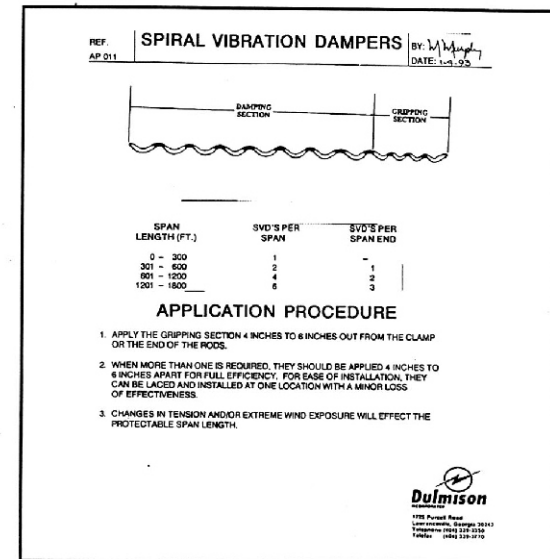
Figure 21 Dulmison spiral vibration damper recommendations
