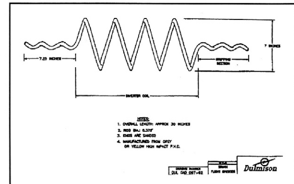
Figure 19 Swan flight diverter (SFD)
