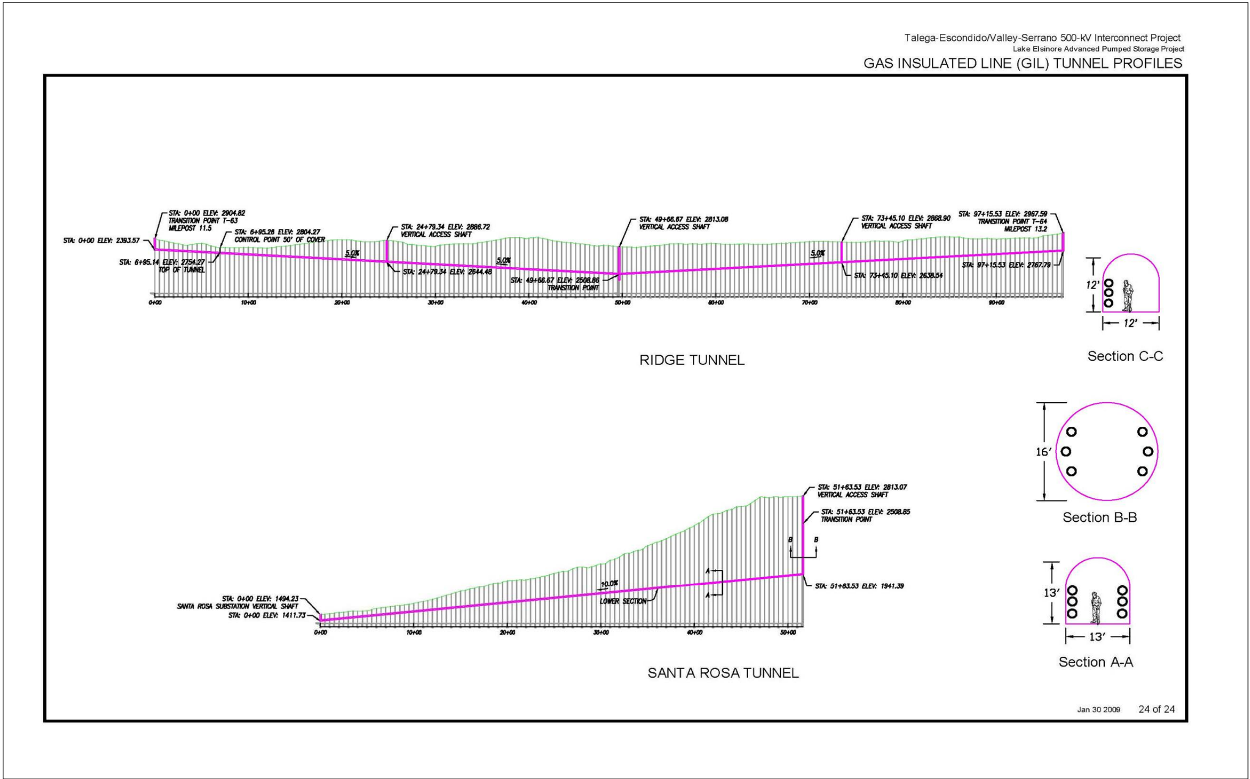
Figure 3.1.1-4: (24 of 24) Talega-Escondido/Valley-Serrano 500 kV Interconnect Project Source: The Nevada Hydro Company
