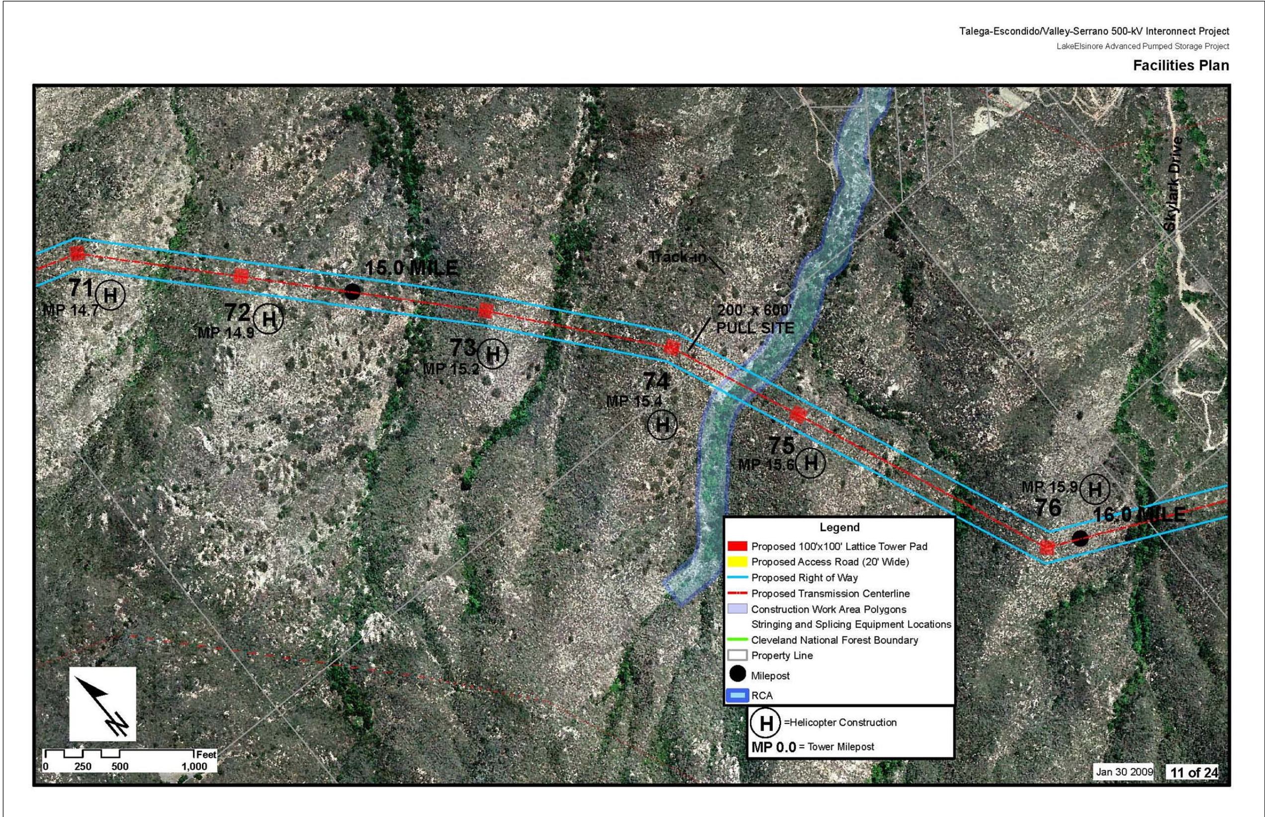
Figure 3.1.1-4: (11 of 24) Talega-Escondido/Valley-Serrano 500 kV Interconnect Project Source: The Nevada Hydro Company
