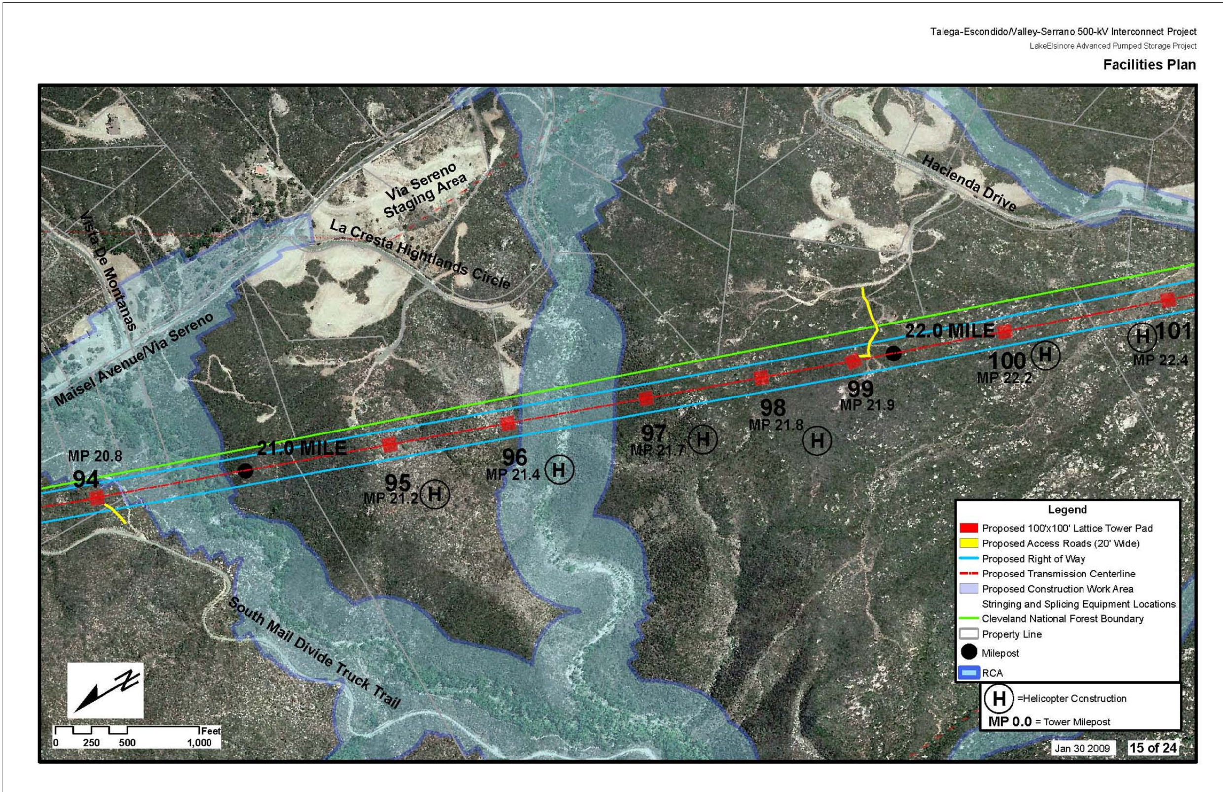
Figure 3.1.1-4: (15 of 24) Talega-Escondido/Valley-Serrano 500 kV Interconnect Project Source: The Nevada Hydro Company
