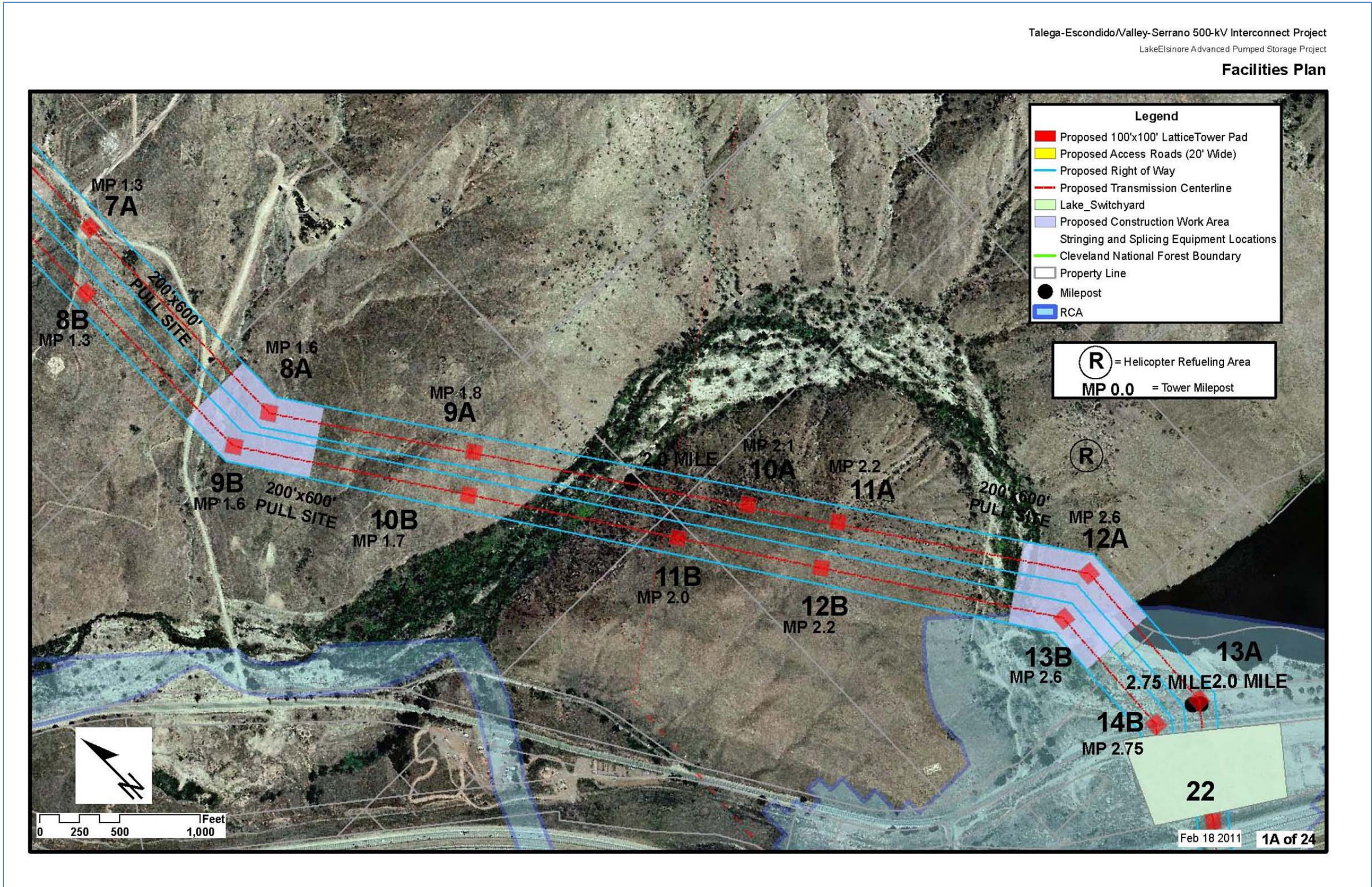
Figure 3.1.1-4: (1A of 24) Talega-Escondido/Valley-Serrano 500 kV Interconnect Project Source: The Nevada Hydro Company
