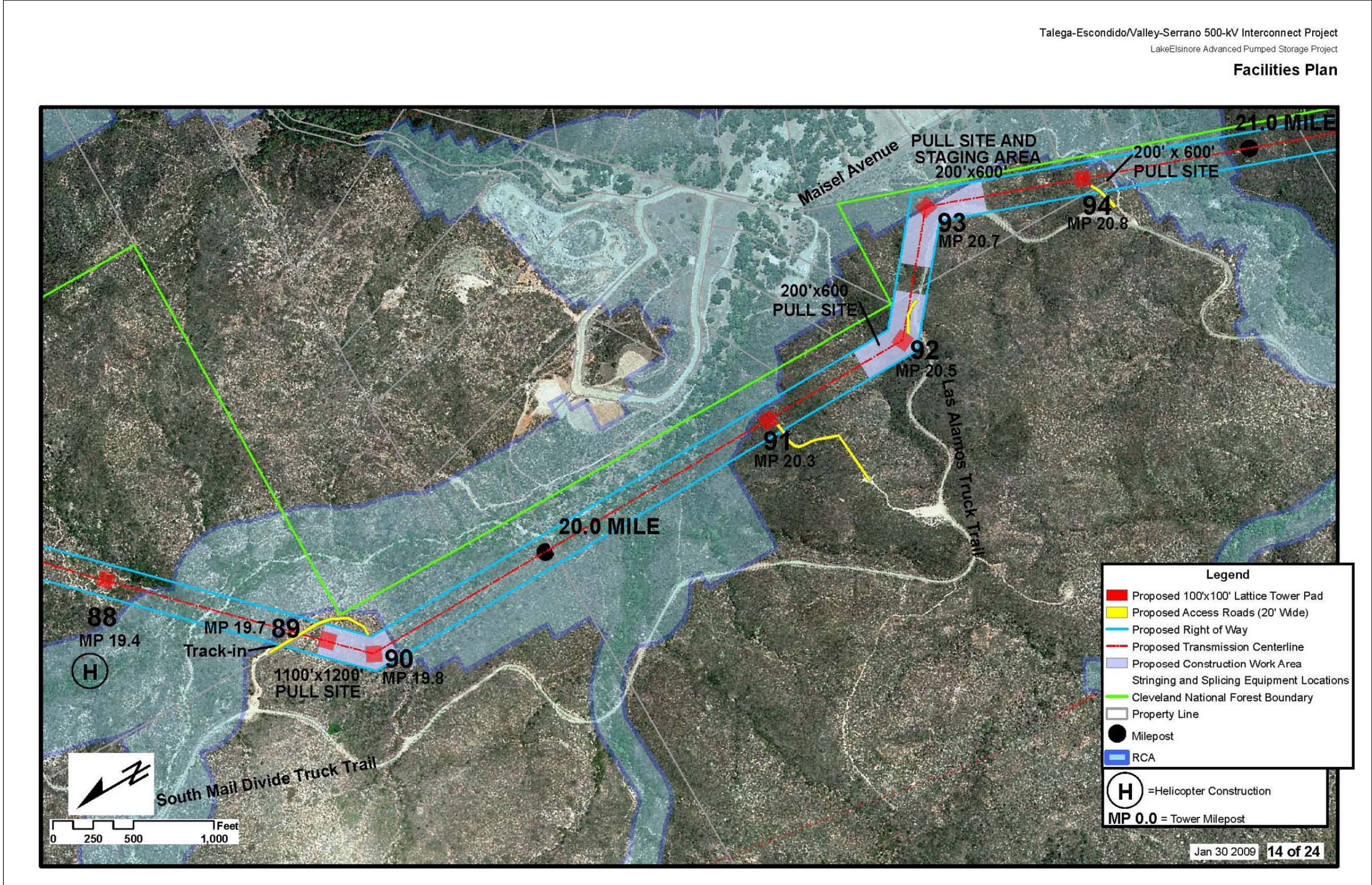
Figure 3.1.1-4: (14 of 24) Talega-Escondido/Valley-Serrano 500 kV Interconnect Project Source: The Nevada Hydro Company
