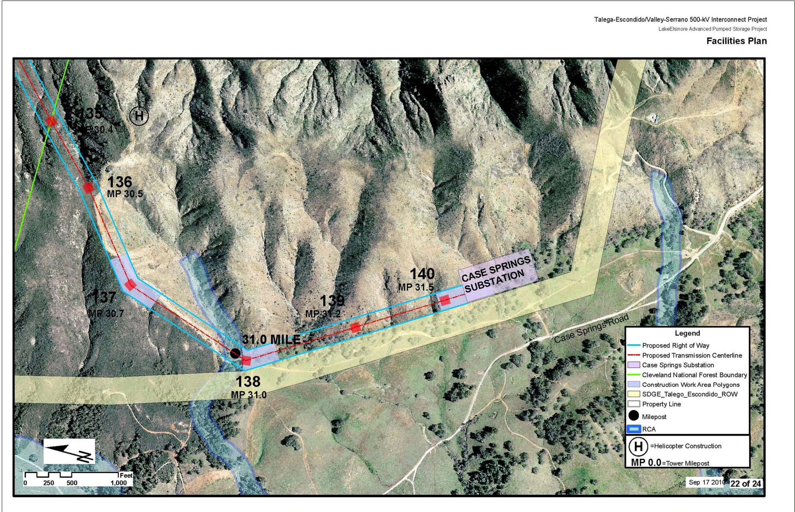
Figure 3.1.1-4: (22 of 24) Talega-Escondido/Valley-Serrano 500 kV Interconnect Project Source: The Nevada Hydro Company
