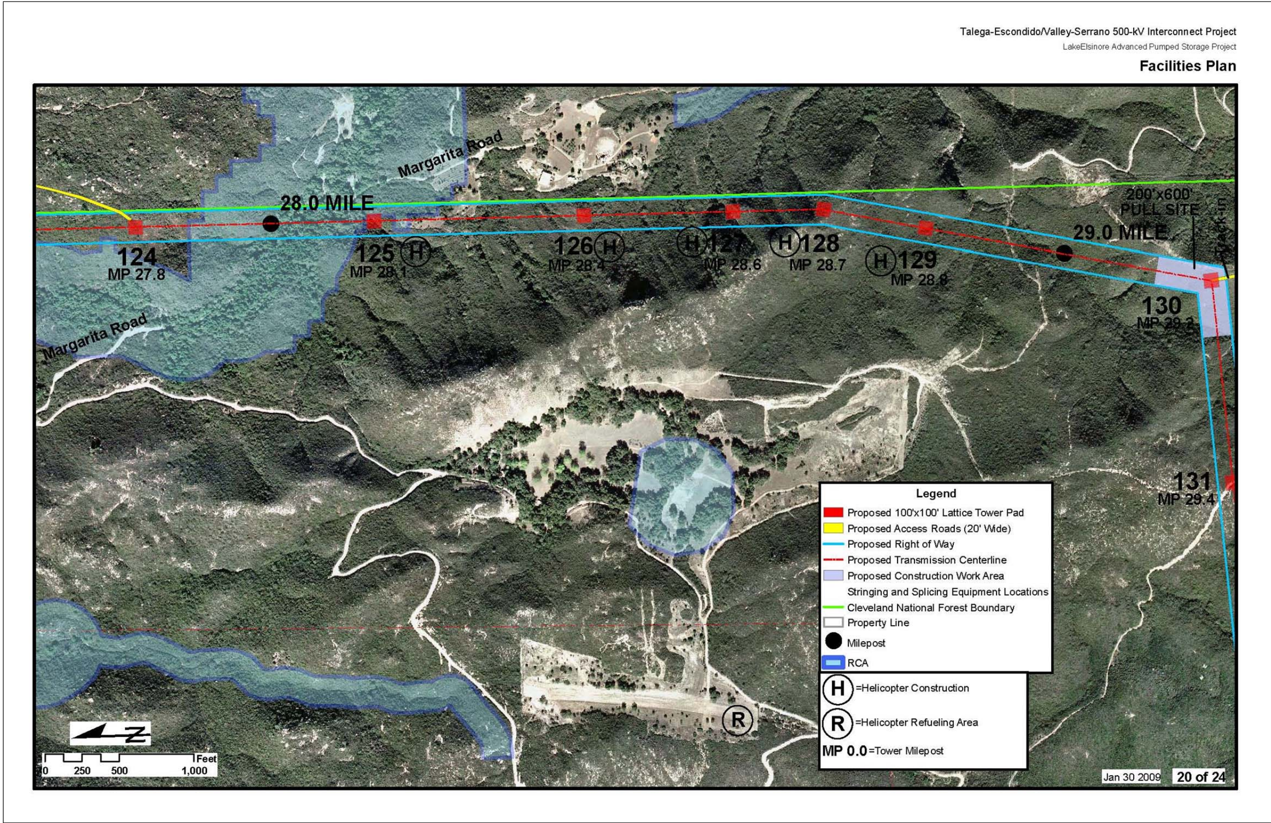
Figure 3.1.1-4: (20 of 24) Talega-Escondido/Valley-Serrano 500 kV Interconnect Project Source: The Nevada Hydro Company
