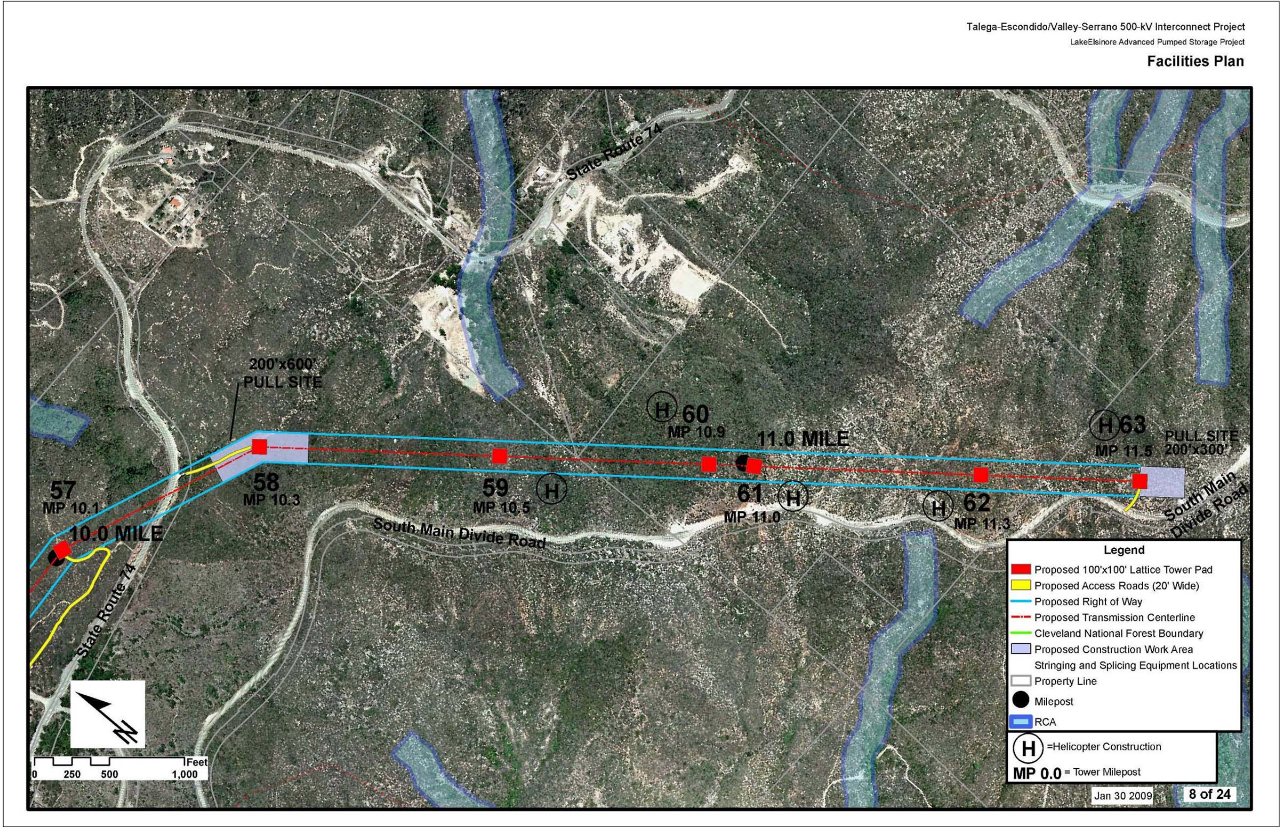
Figure 3.1.1-4: (8 of 24) Talega-Escondido/Valley-Serrano 500 kV Interconnect Project Source: The Nevada Hydro Company
