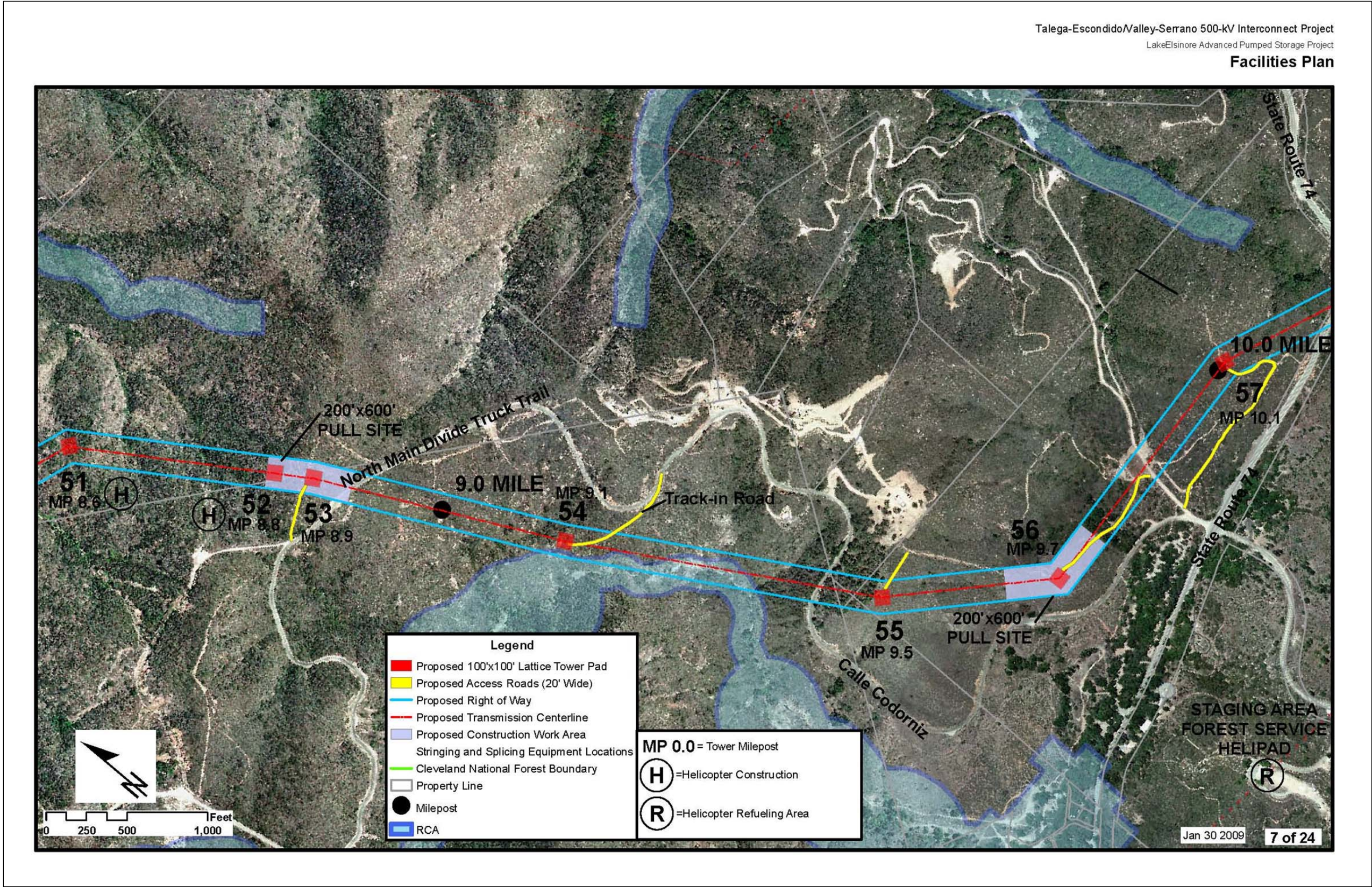
Figure 3.1.1-4: (7 of 24) Talega-Escondido/Valley-Serrano 500 kV Interconnect Project Source: The Nevada Hydro Company
