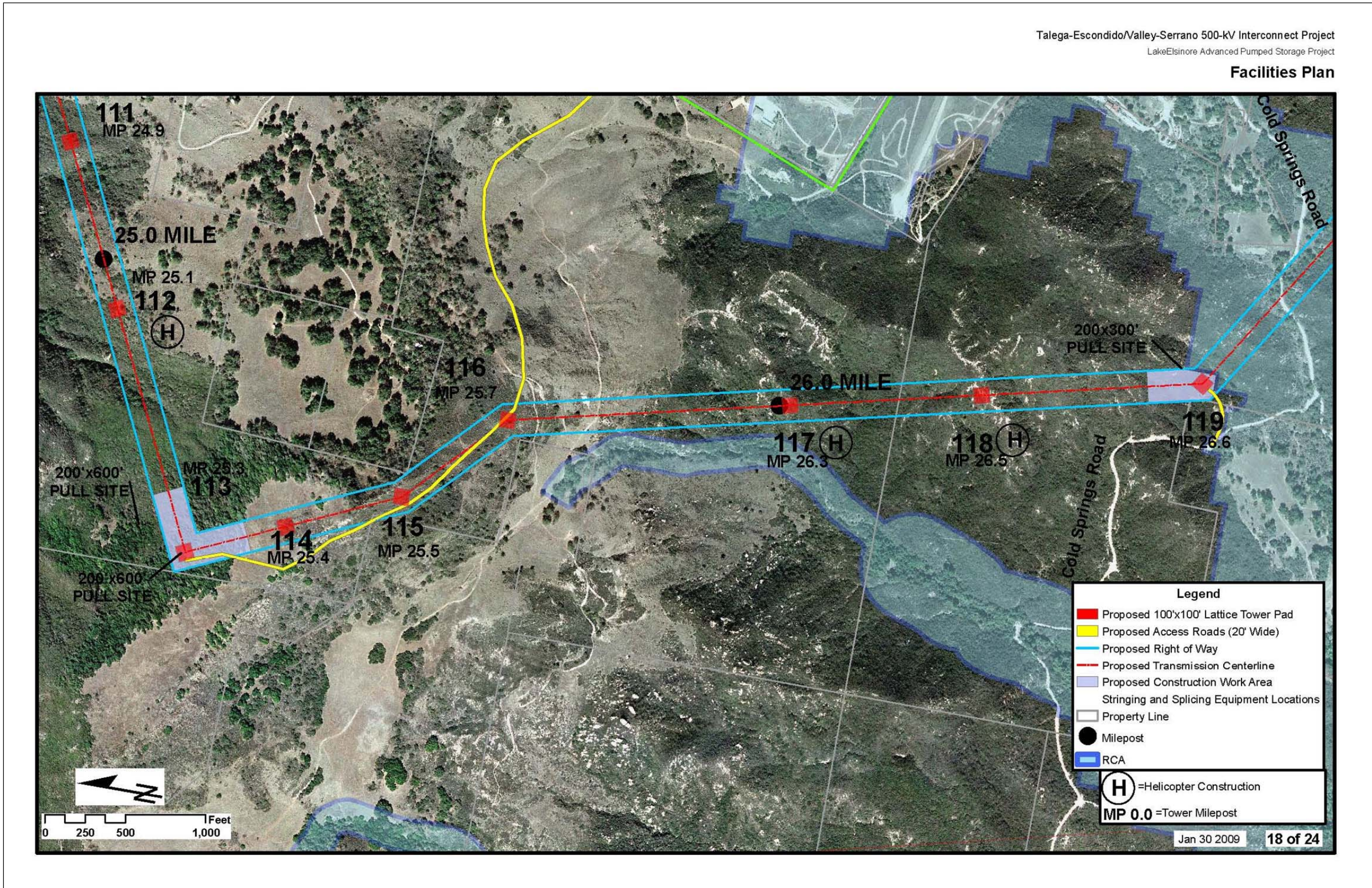
Figure 3.1.1-4: (18 of 24) Talega-Escondido/Valley-Serrano 500 kV Interconnect Project Source: The Nevada Hydro Company
