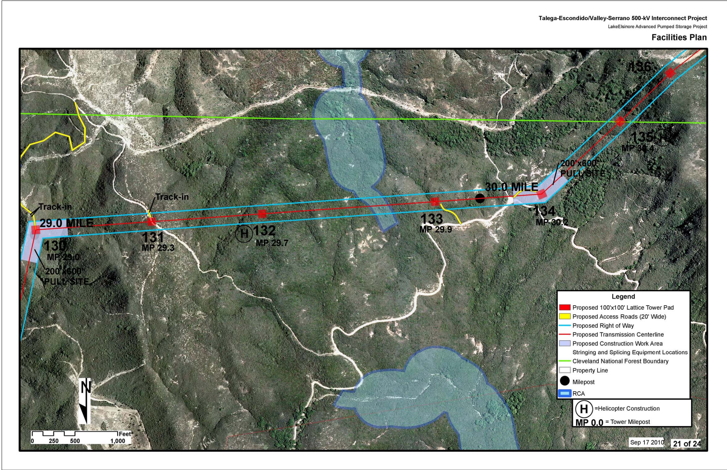
Figure 3.1.1-4: (21 of 24) Talega-Escondido/Valley-Serrano 500 kV Interconnect Project
