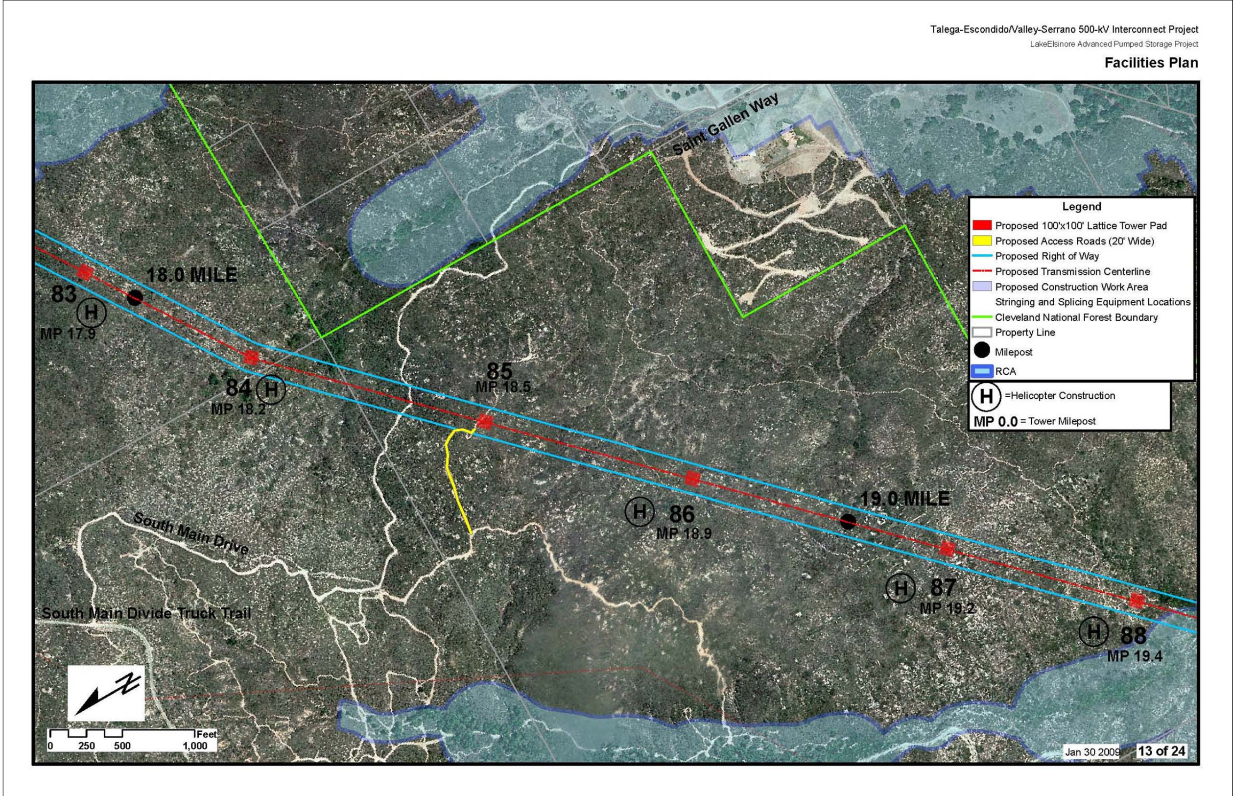
Figure 3.1.1-4: (13 of 24) Talega-Escondido/Valley-Serrano 500 kV Interconnect Project Source: The Nevada Hydro Company
