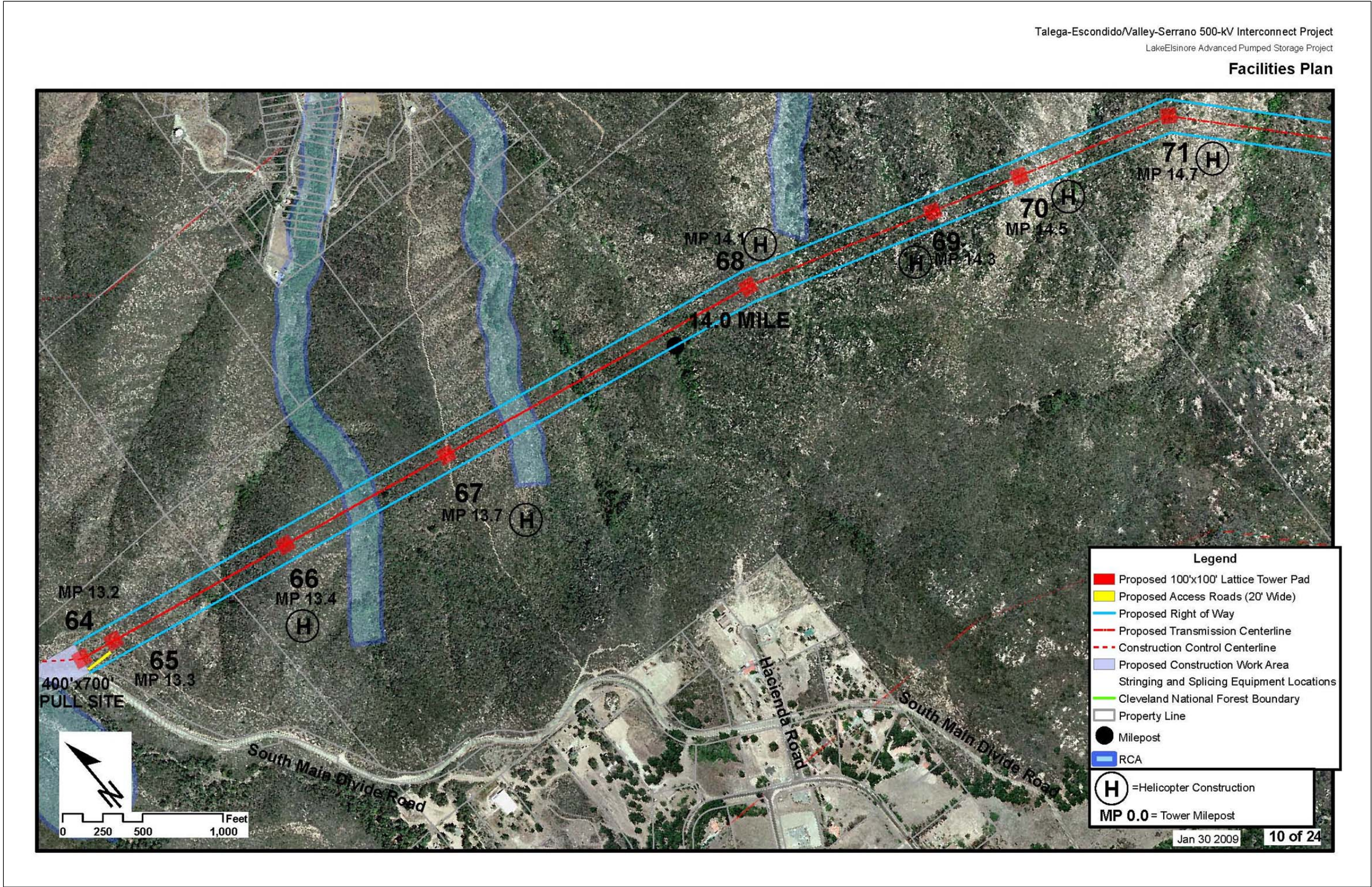
Figure 3.1.1-4: (10 of 24) Talega-Escondido/Valley-Serrano 500 kV Interconnect Project
