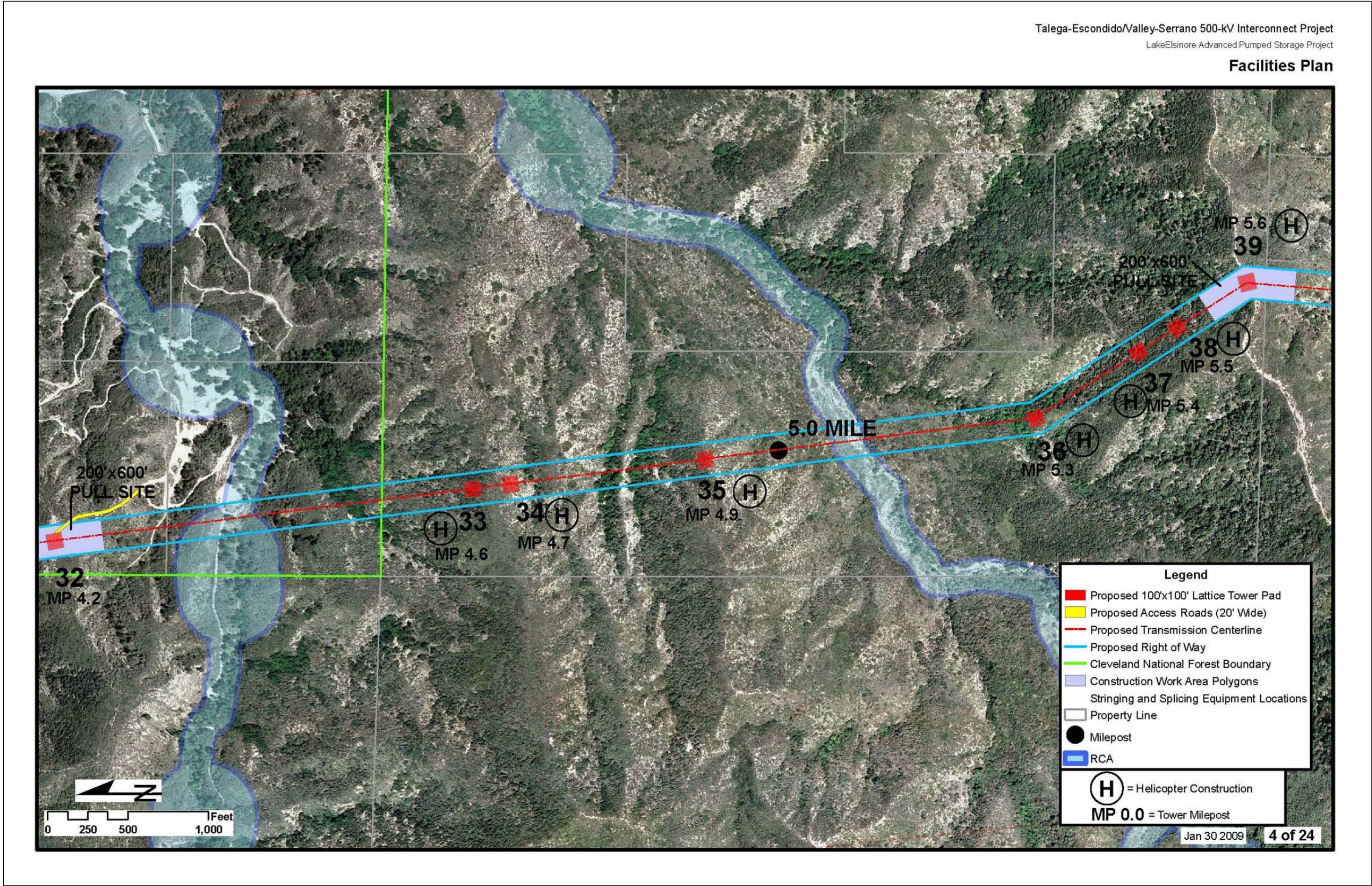
Figure 3.1.1-4: (4 of 24) Talega-Escondido/Valley-Serrano 500 kV Interconnect Project Source: The Nevada Hydro Company
