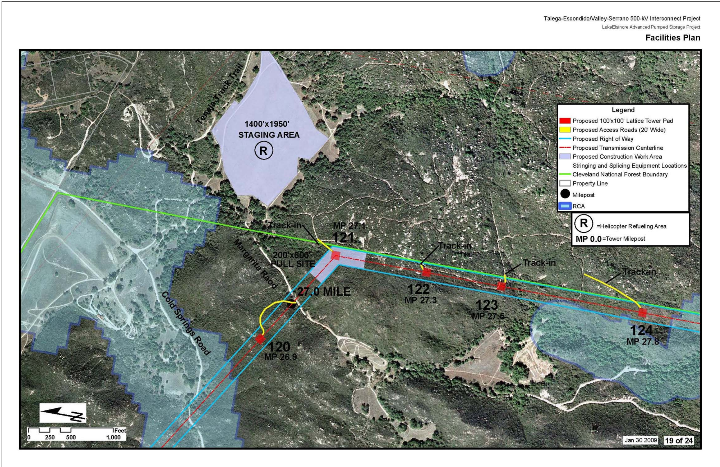
Figure 3.1.1-4: (19 of 24) Talega-Escondido/Valley-Serrano 500 kV Interconnect Project Source: The Nevada Hydro Company
