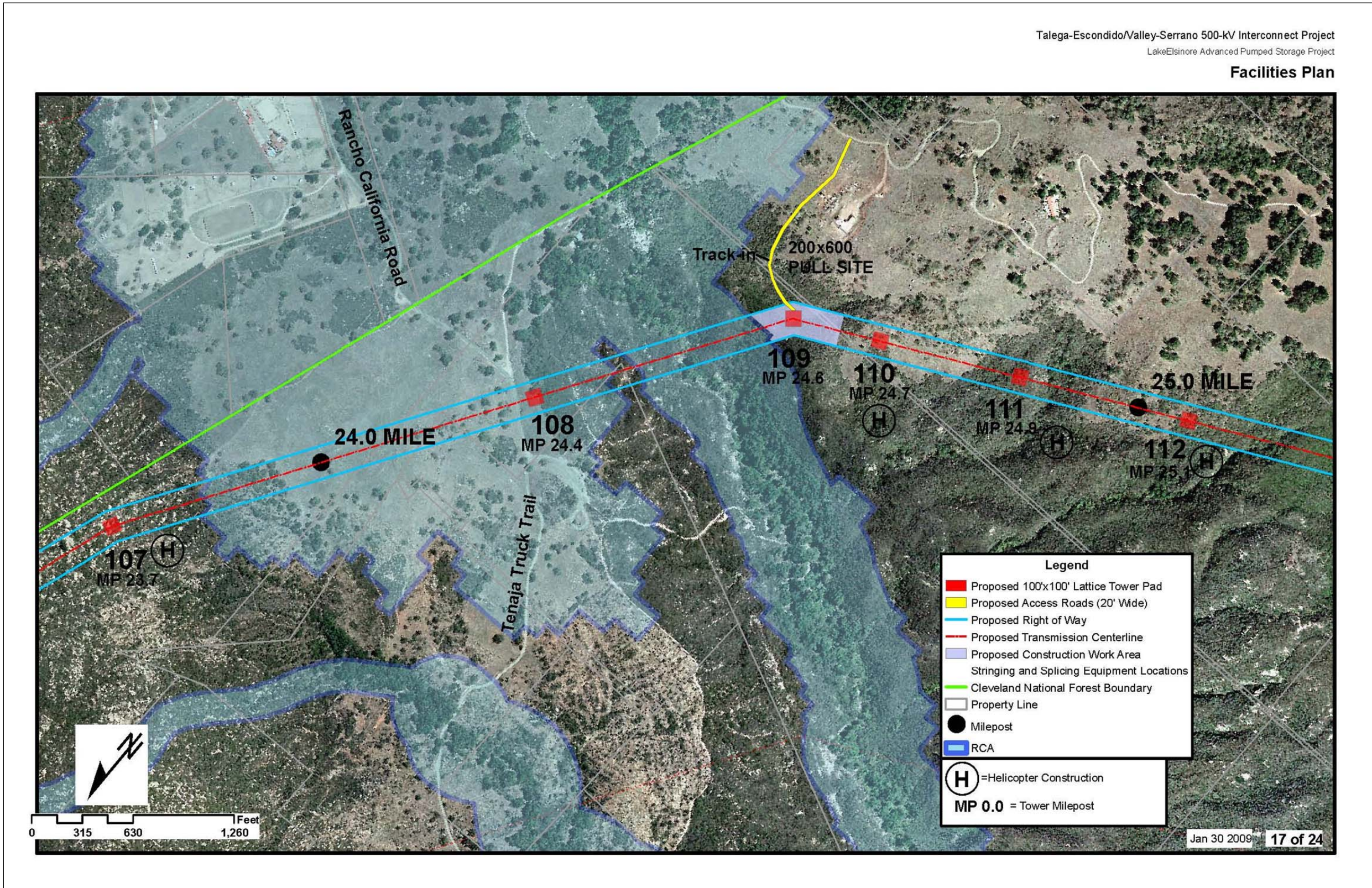
Figure 3.1.1-4: (17 of 24) Talega-Escondido/Valley-Serrano 500 kV Interconnect Project Source: The Nevada Hydro Company
