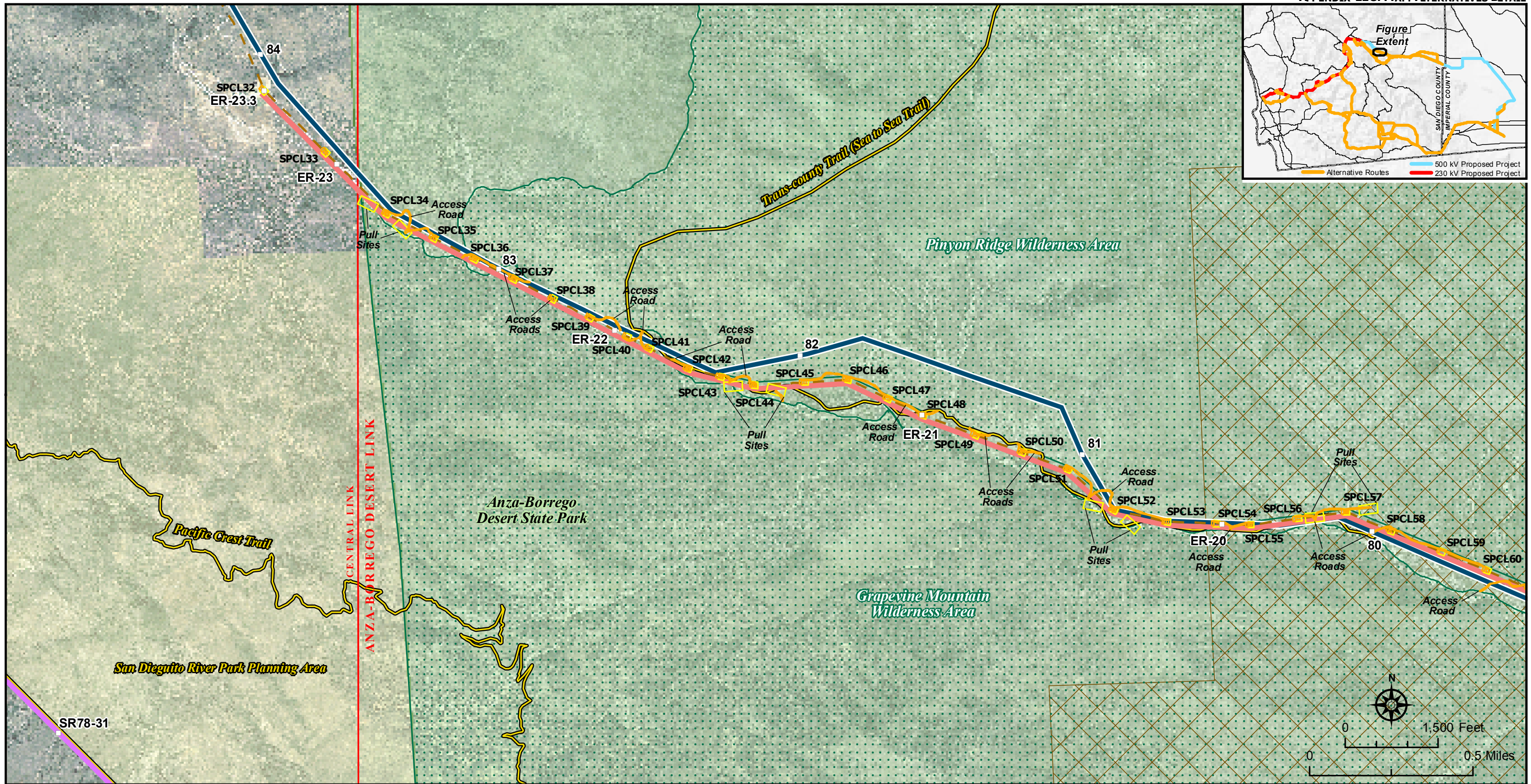
Sunrise Powerlink Project Figure Ap. 11C-18 Overhead 500 kV ABDSP Within Existing ROW Alternative Detail
