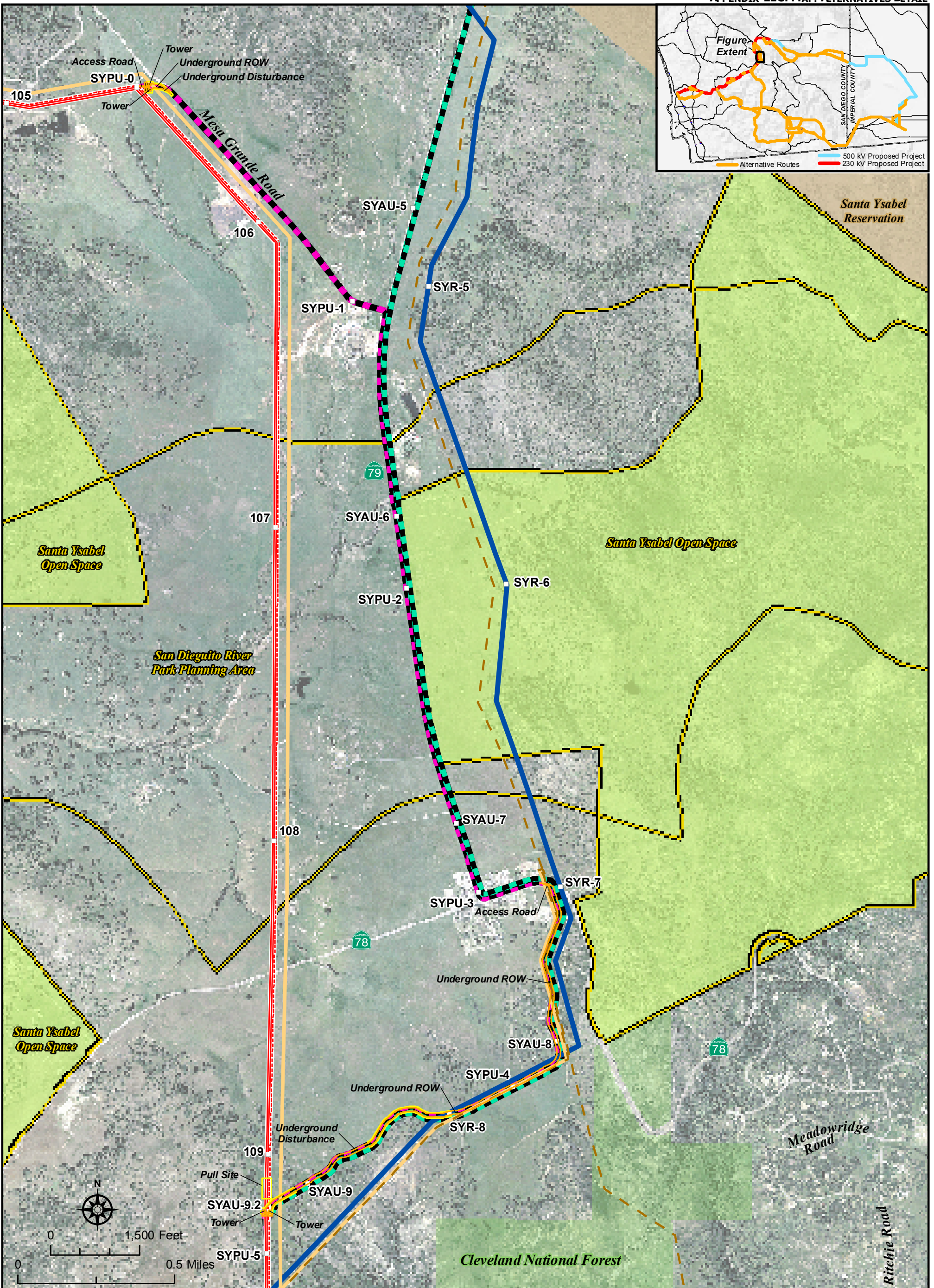
Sunrise Powerlink Project Figure Ap. 11C-21 Santa Ysabel Partial Underground Alternative Detail
