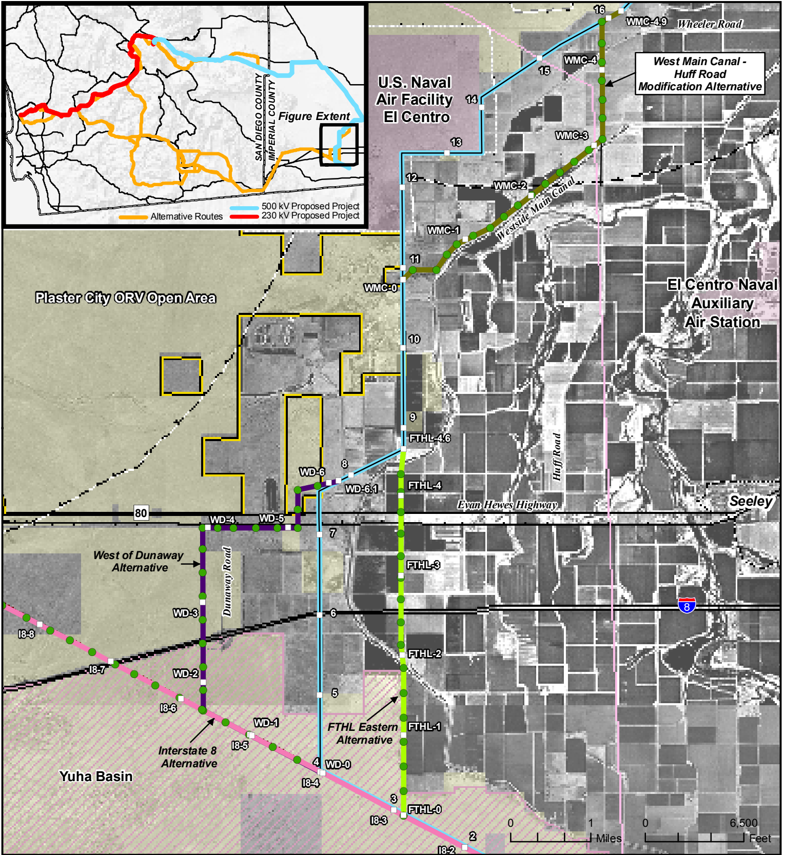
Sunrise Powerlink Project Figure Ap.1-2 Imperial Valley Link: Alternatives Retained
