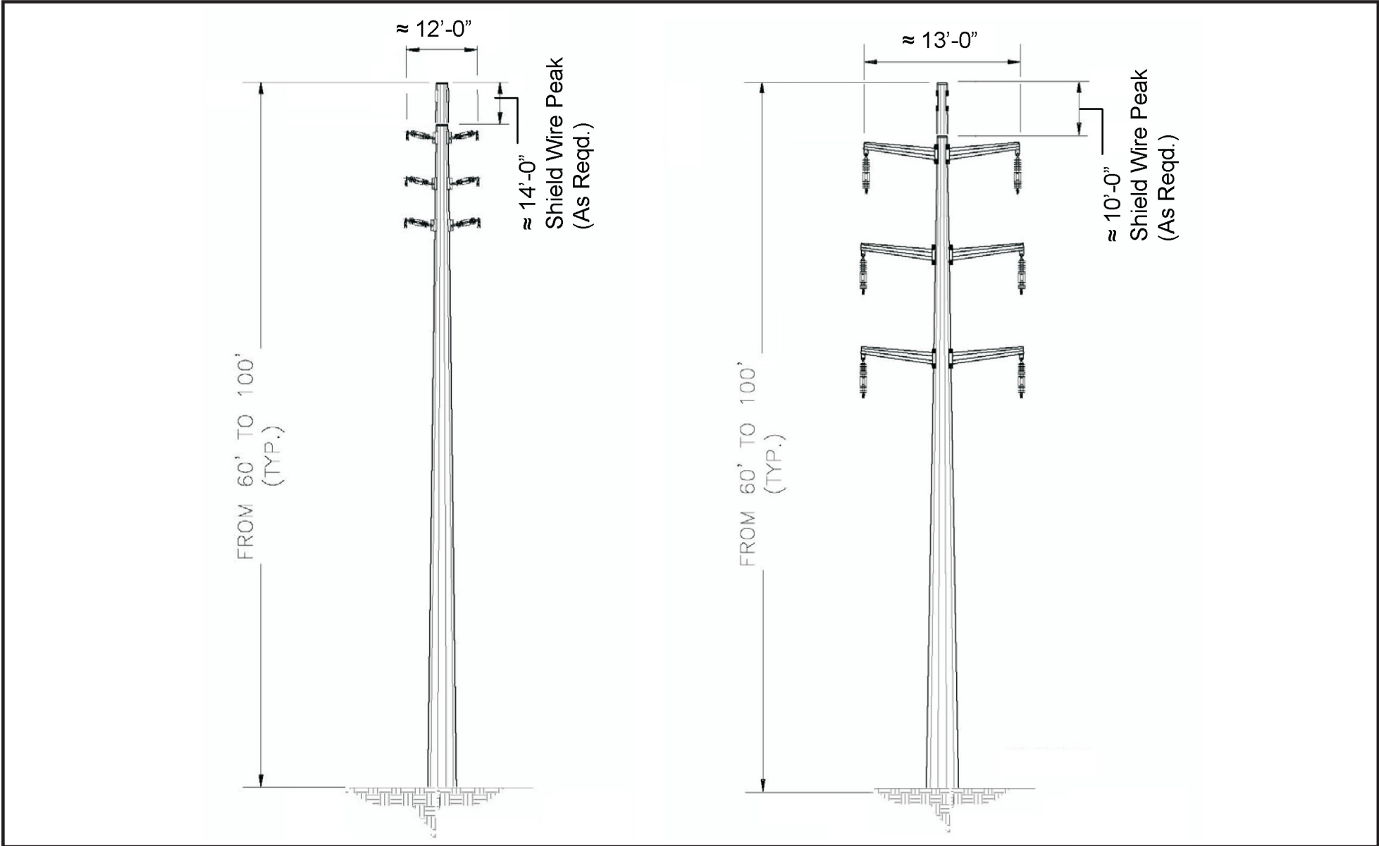
Figure Ap. 1-9 SDG&E 100-Foot ROW Shorter Structure Alternative - Typical 69 kV Poles
