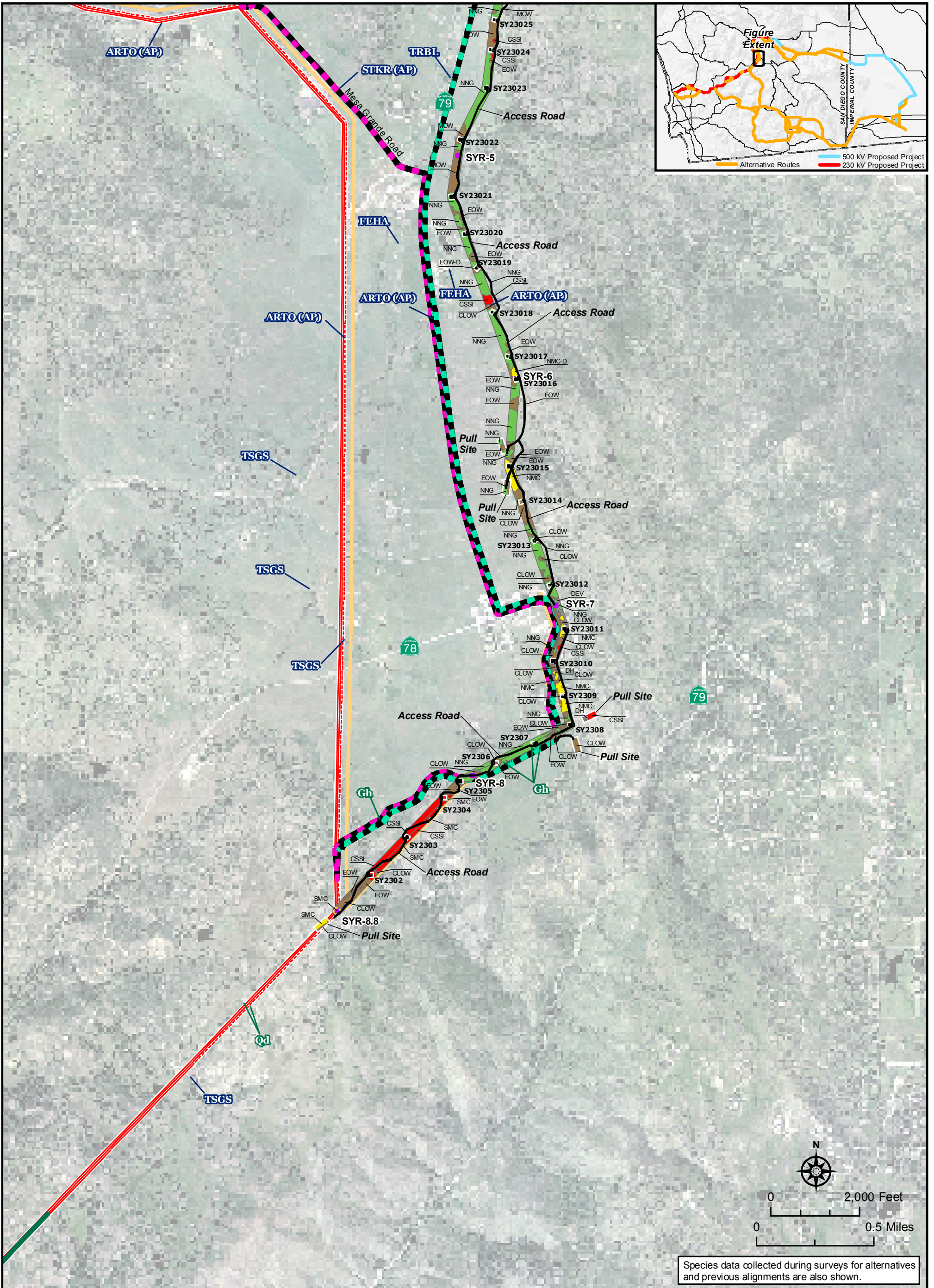
Sunrise Powerlink Project Figure Ap. 8F-2 Santa Ysabel Existing ROW Alternative Biological Resources/Impacts
