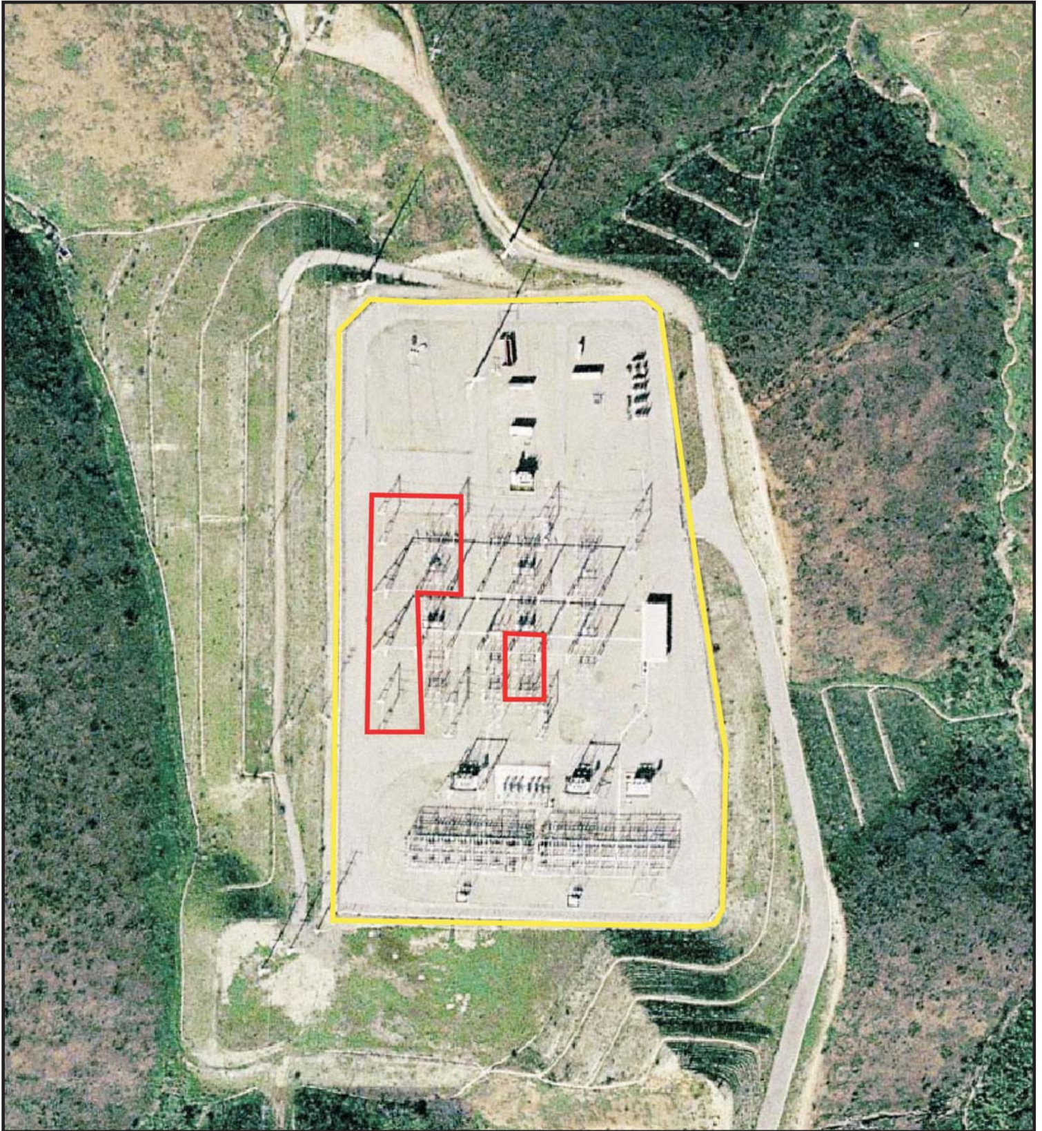
Figure B-38 Sycamore Canyon Substation: Proposed Modifications
