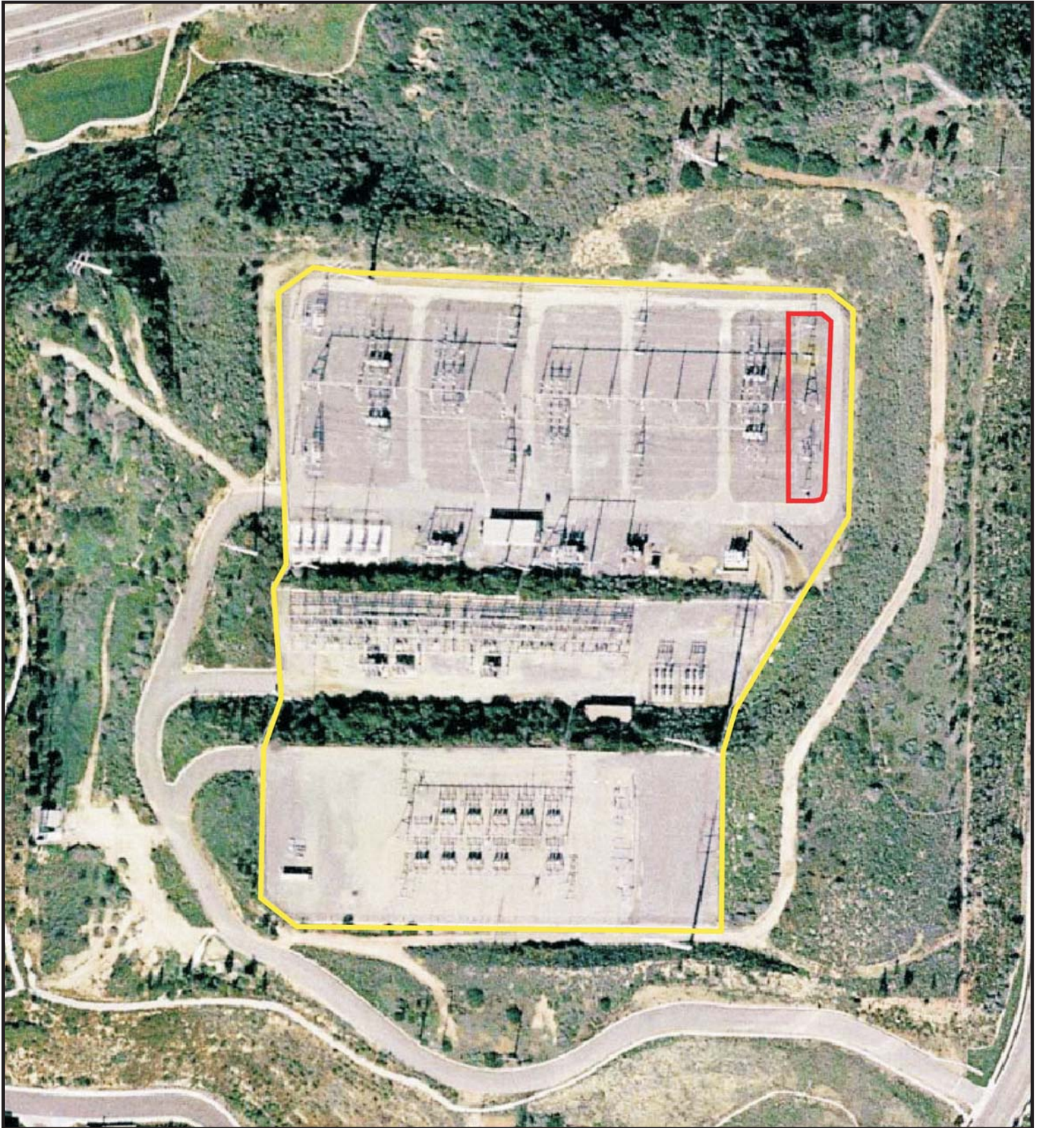
Figure B-39 Penasquitos Substation: Proposed Modifications
