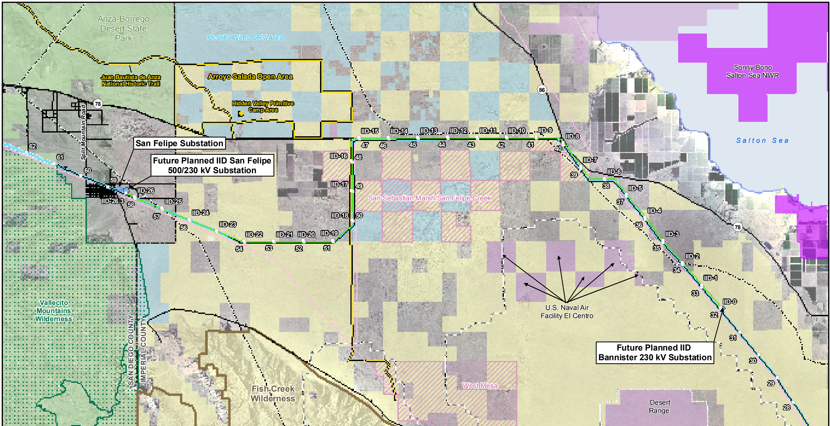
Sunrise Powerlink Project Figure B-45 Connected Actions: IID Transmission System Upgrades
