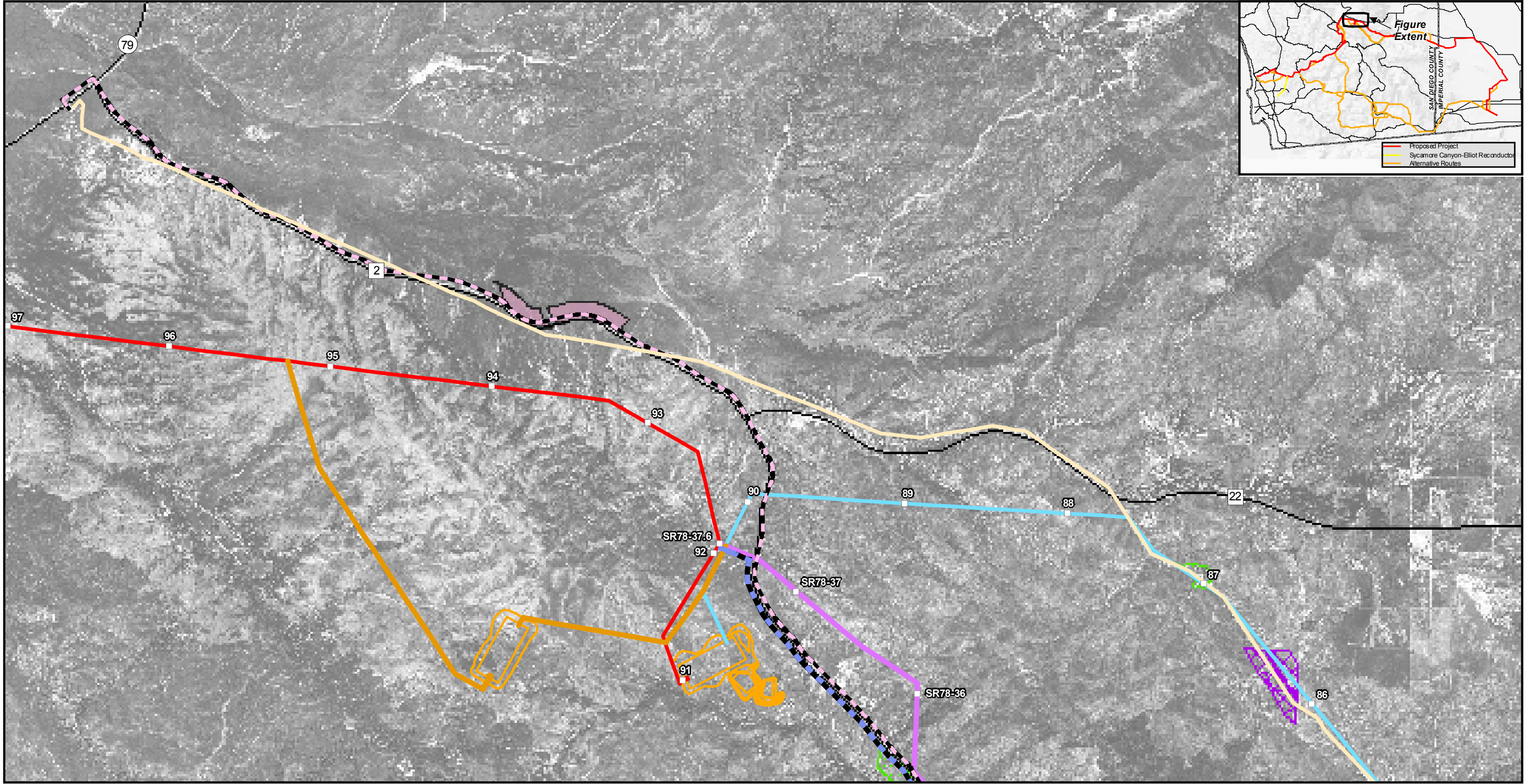
Sunrise Powerlink Project Figure Ap.AG E.5-5 Agriculture: New In-Area Renewable Generation, Solar Thermal: Narrows-Warners 138 kV Upgrade Options
