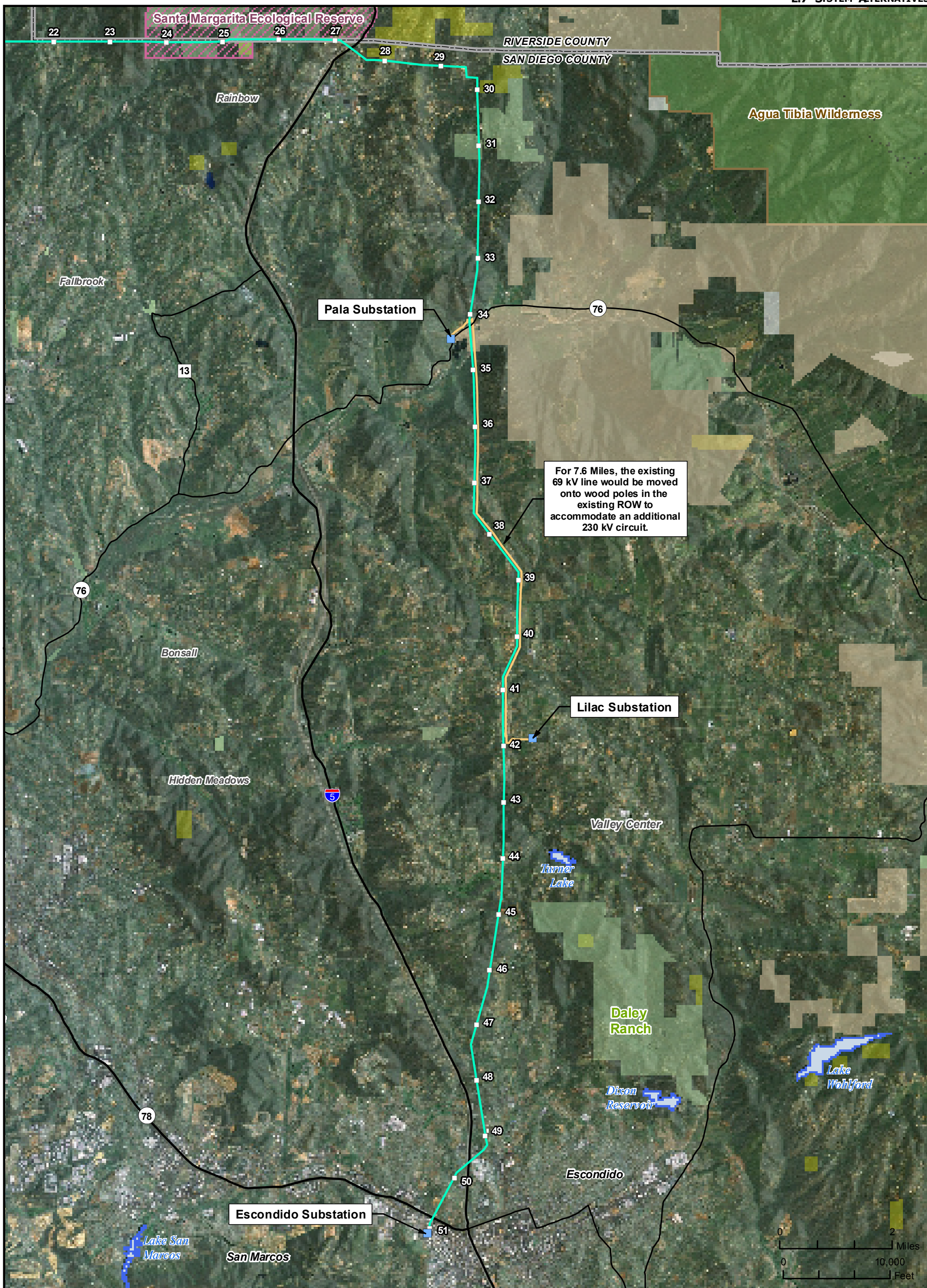
Sunrise Powerlink Project Figure E.7.1-2d LEAPS Transmission-Only Alternative: Pala to Escondido
