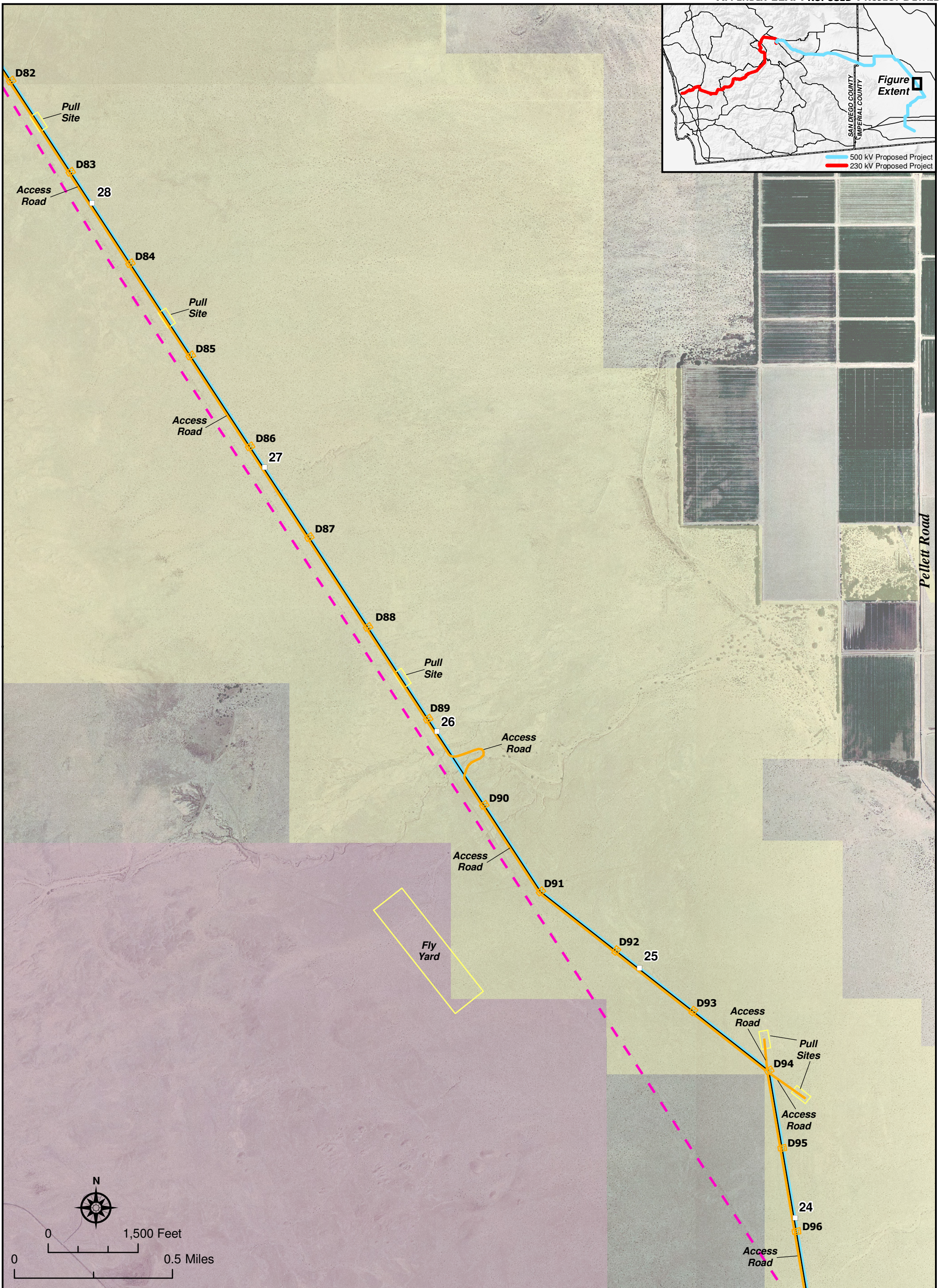
Sunrise Powerlink Project Figure Ap. 11A-7 Proposed Project Detail
