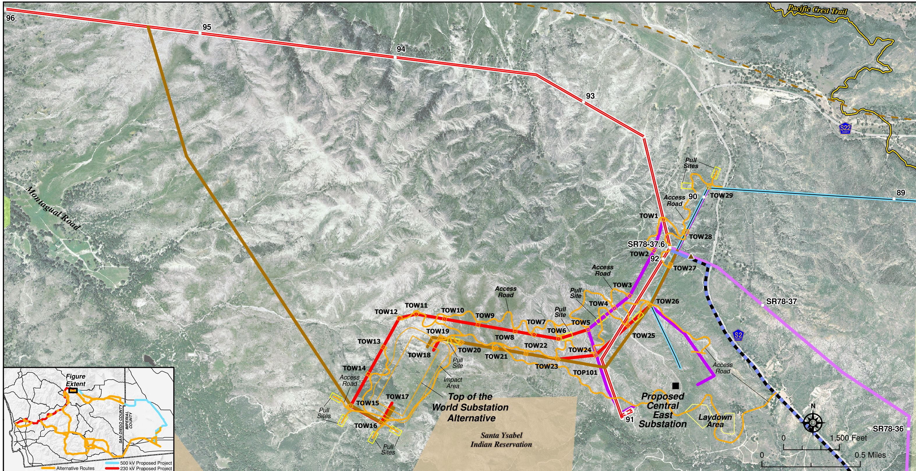
Sunrise Powerlink Project Figure Ap. 11C-34 Top of the World Substation Alternative Detail
