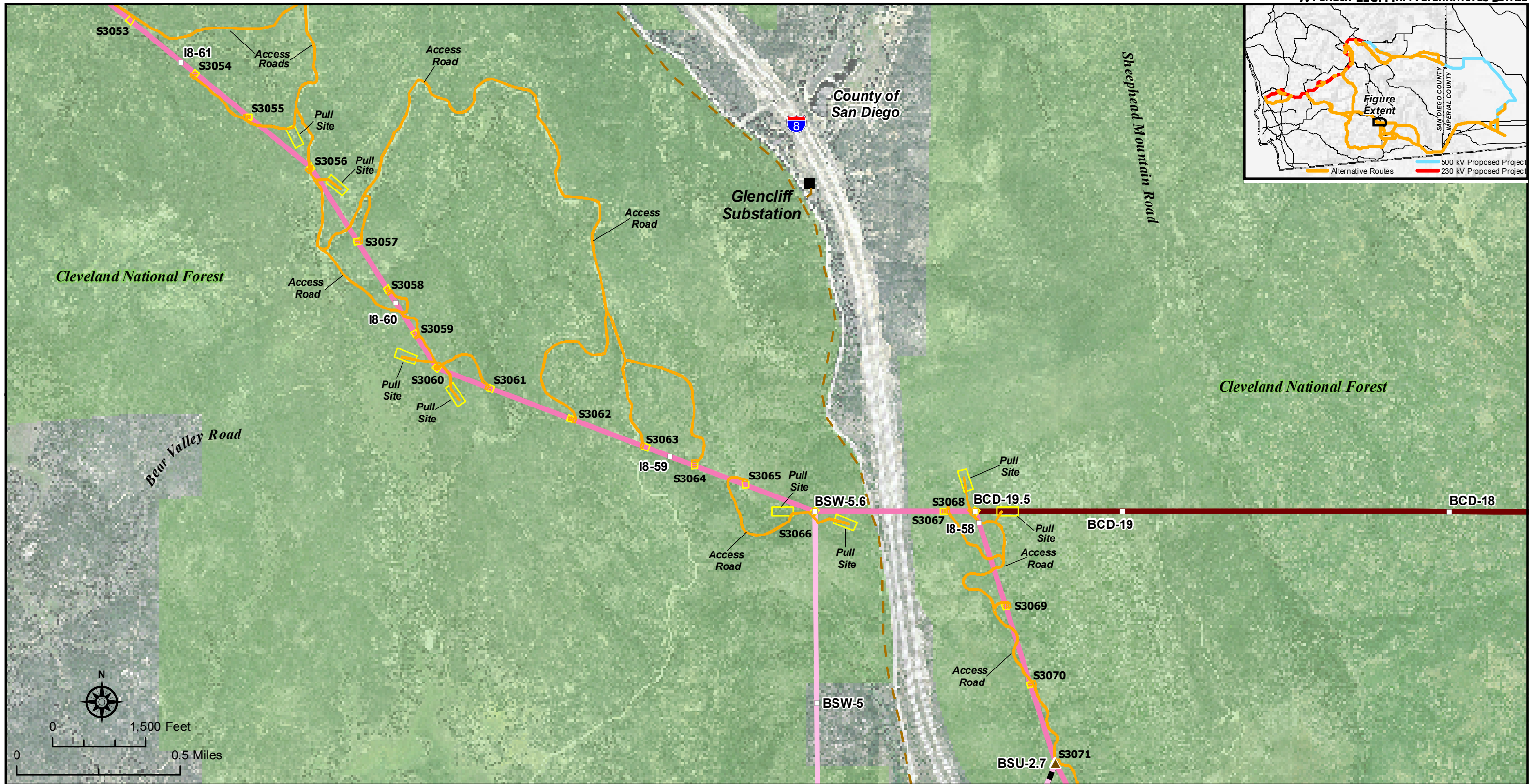
Sunrise Powerlink Project Figure Ap. 11C-49 Interstate 8 Alternative, Overhead Portion Detail
