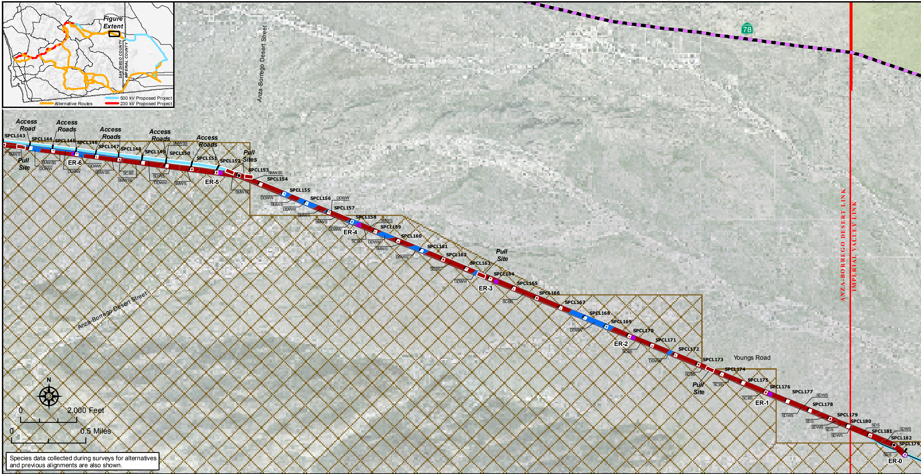
Sunrise Powerlink Project Figure Ap. 8E-7 Overhead 500 kV ABDSP Within Existing ROW Alternative Biological Resources/Impacts
