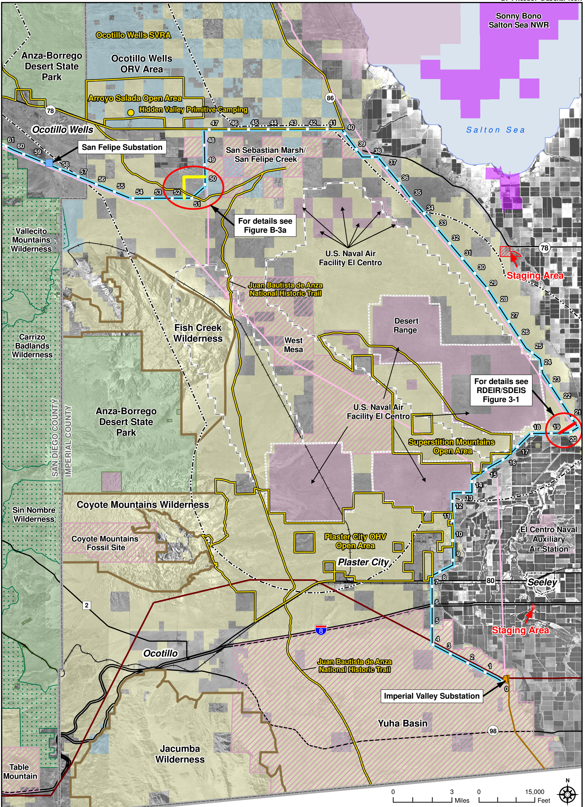
Sunrise Powerlink Project Figure B-3 Imperial Valley Link
