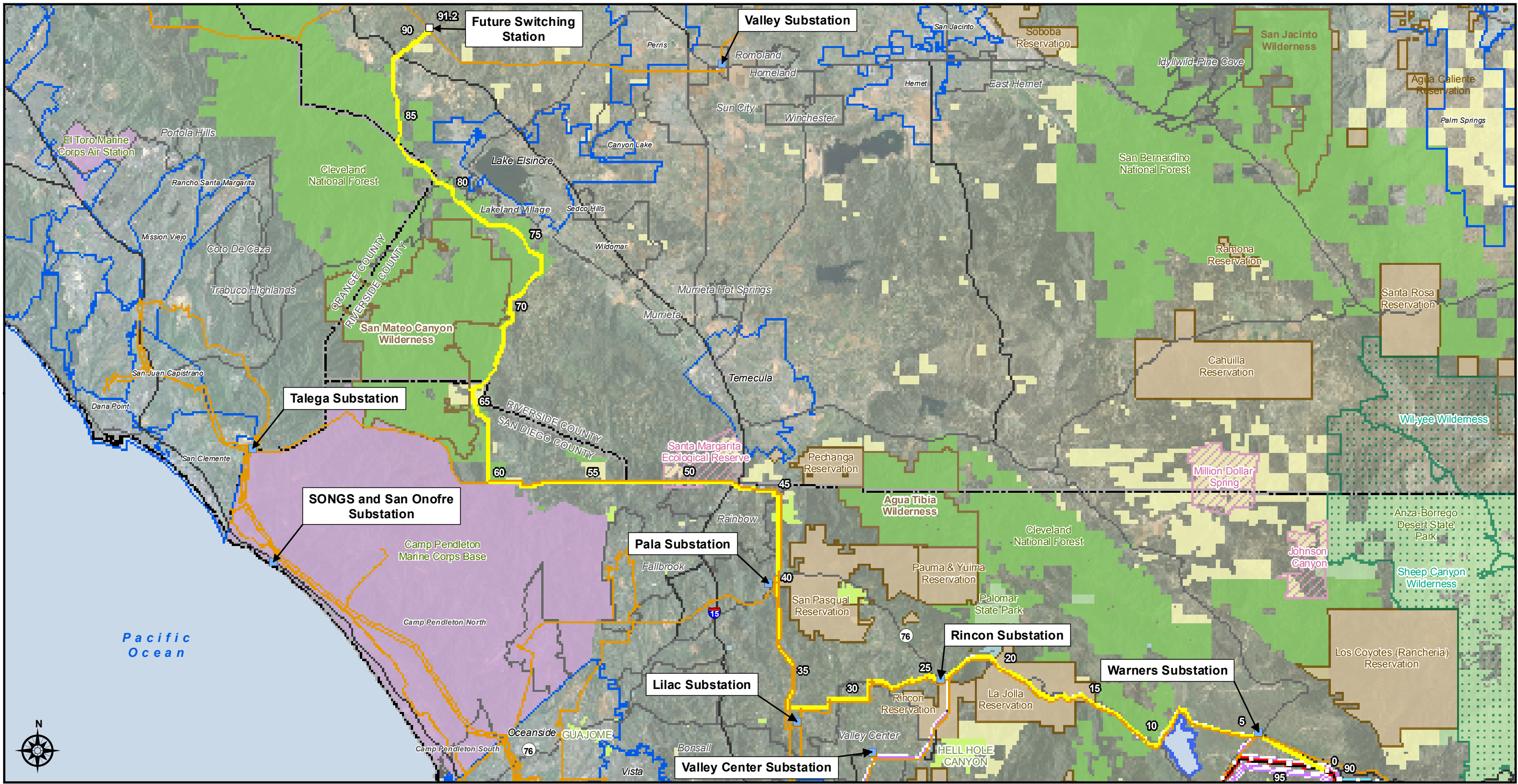
Sunrise Powerlink Project Figure B-12b Future Transmission System Expansion: 500 kV Central East to Riverside
