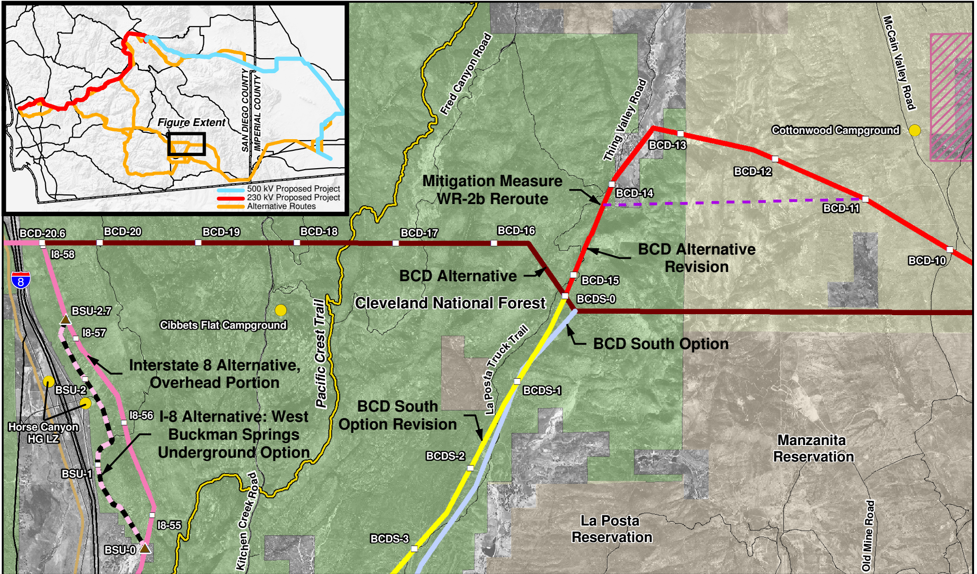
Sunrise Powerlink Project Figure E.2.1-1b BCD Alternative (MPs BCD-10 to 20.6)
