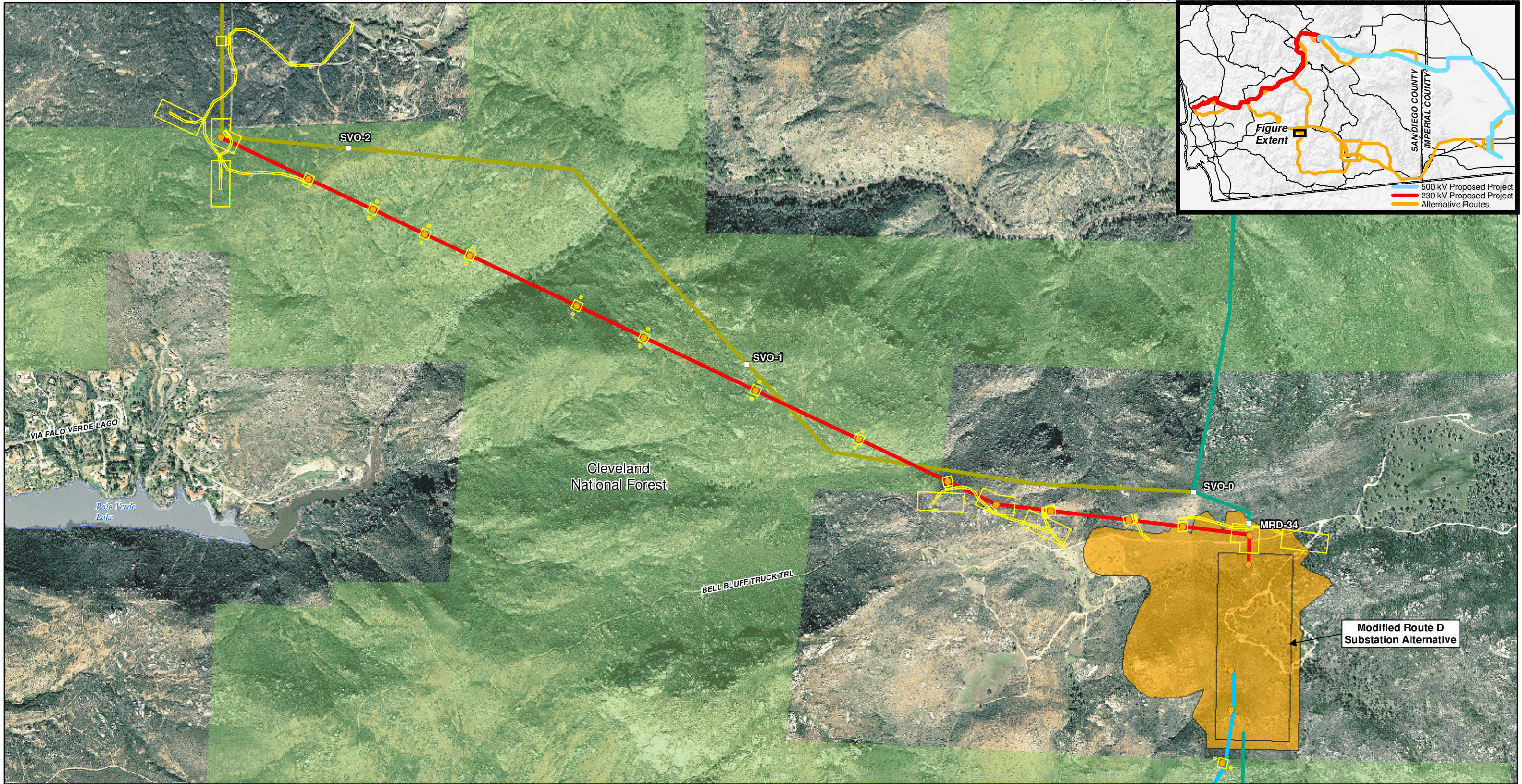
Sunrise Powerlink Project Figure 3-13 Modified Route D Alternative: Star Valley Option Revision
