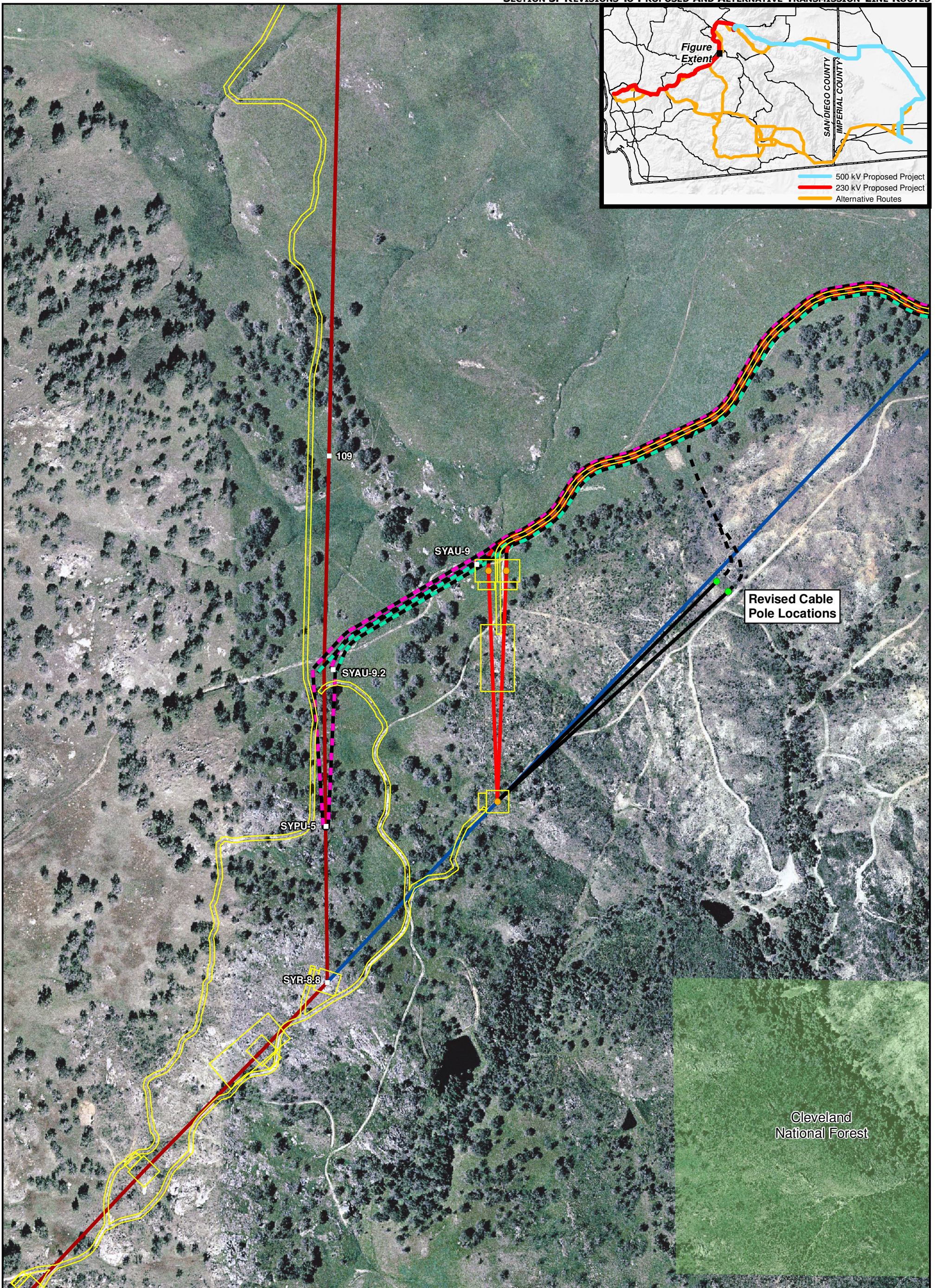
Sunrise Powerlink Project Figure 3-4A Santa Ysabel Partial Underground Alternative Revision: Southern Transition Relocation
