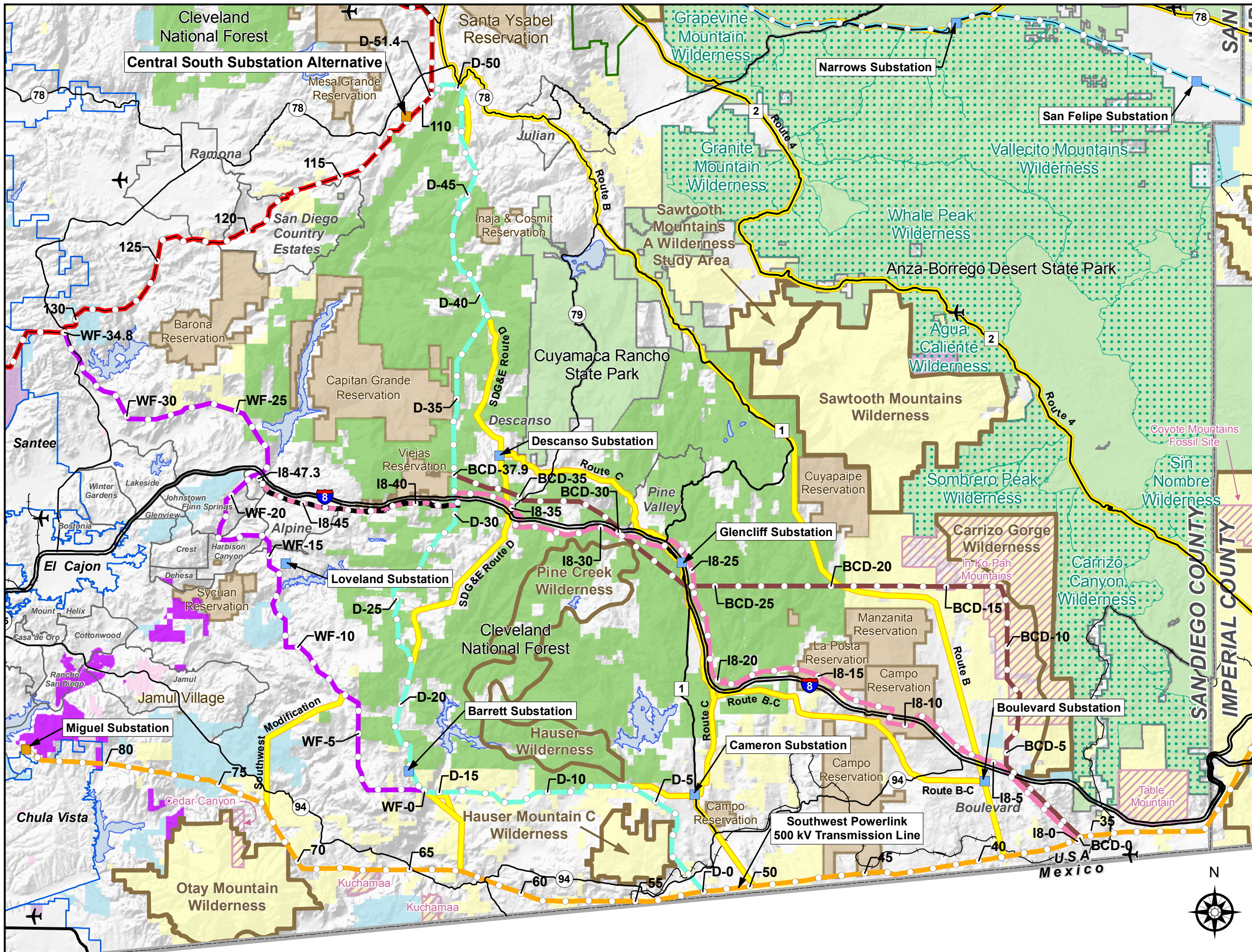
Sunrise Powerlink Project Figure 8 Southwest Powerlink Alternatives
