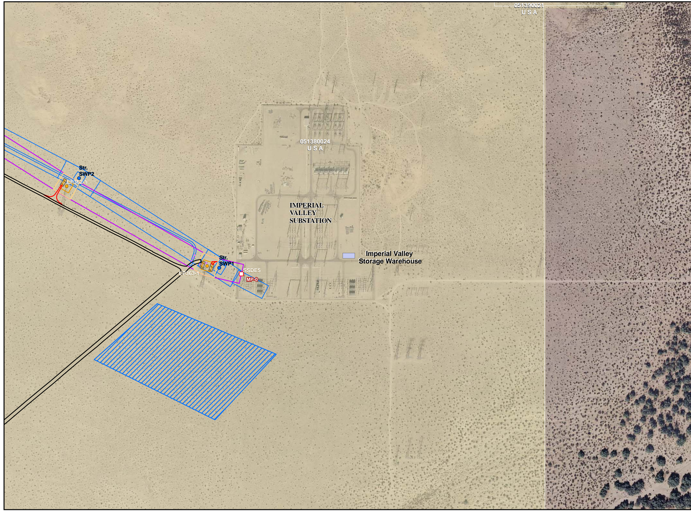
Figure 1 IMPERIAL VALLEY SUBSTATION
