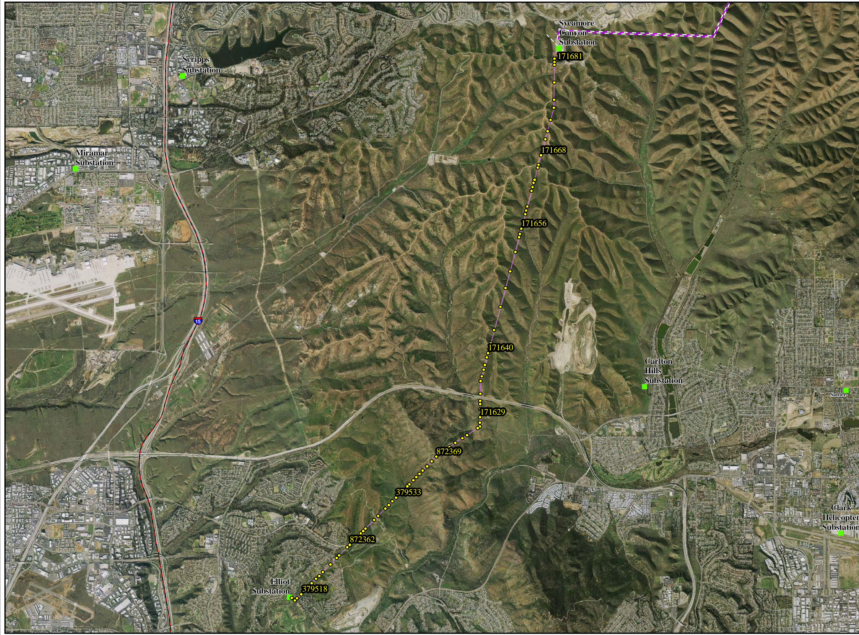
Figure 43 SYCAMORE CANYON - ELLIOTT SUBSTATION RECONDUCTORING PROJECT OVERVIEW
