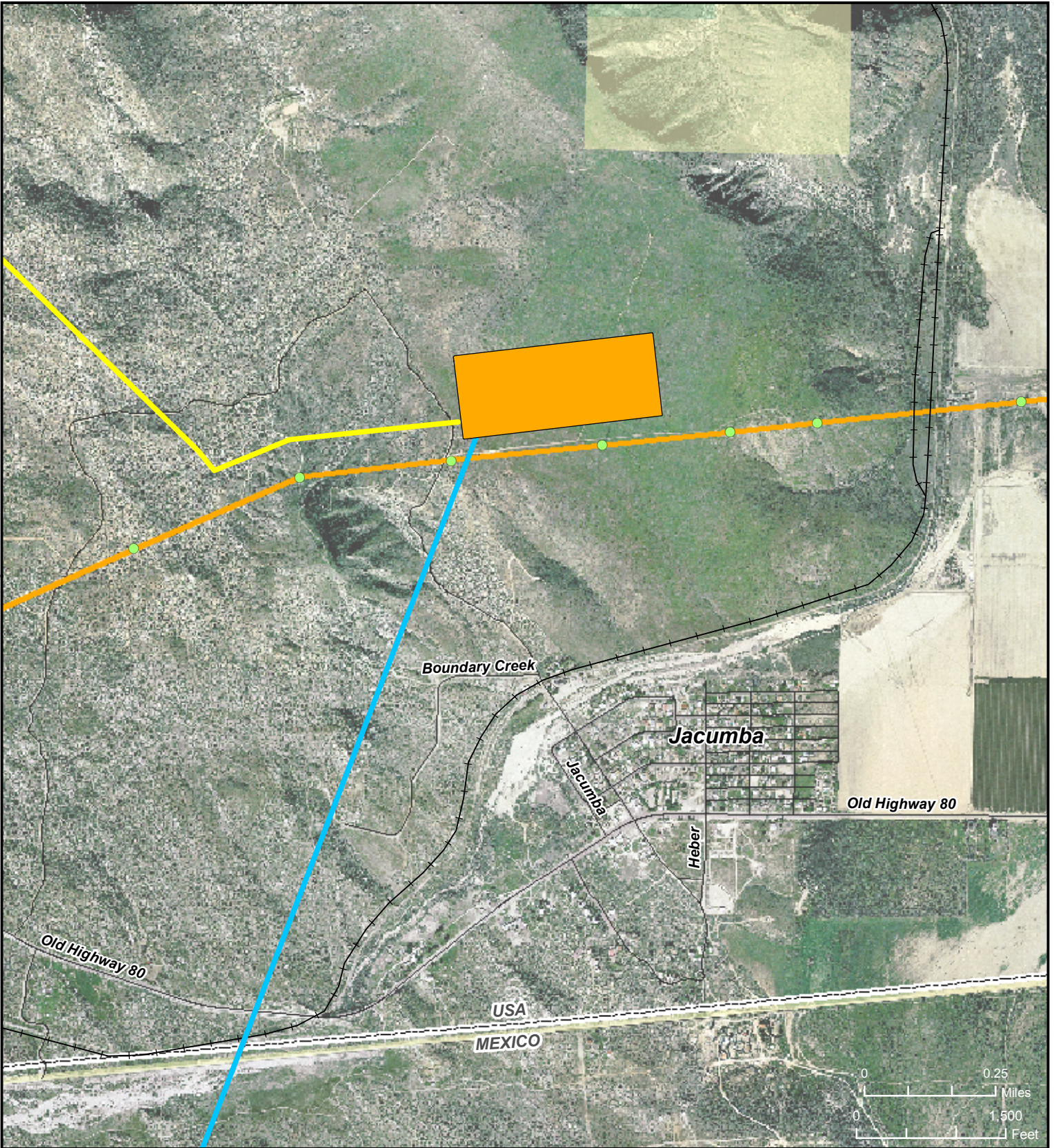
Sunrise Powerlink Project Figure B-47 Jacumba Substation
