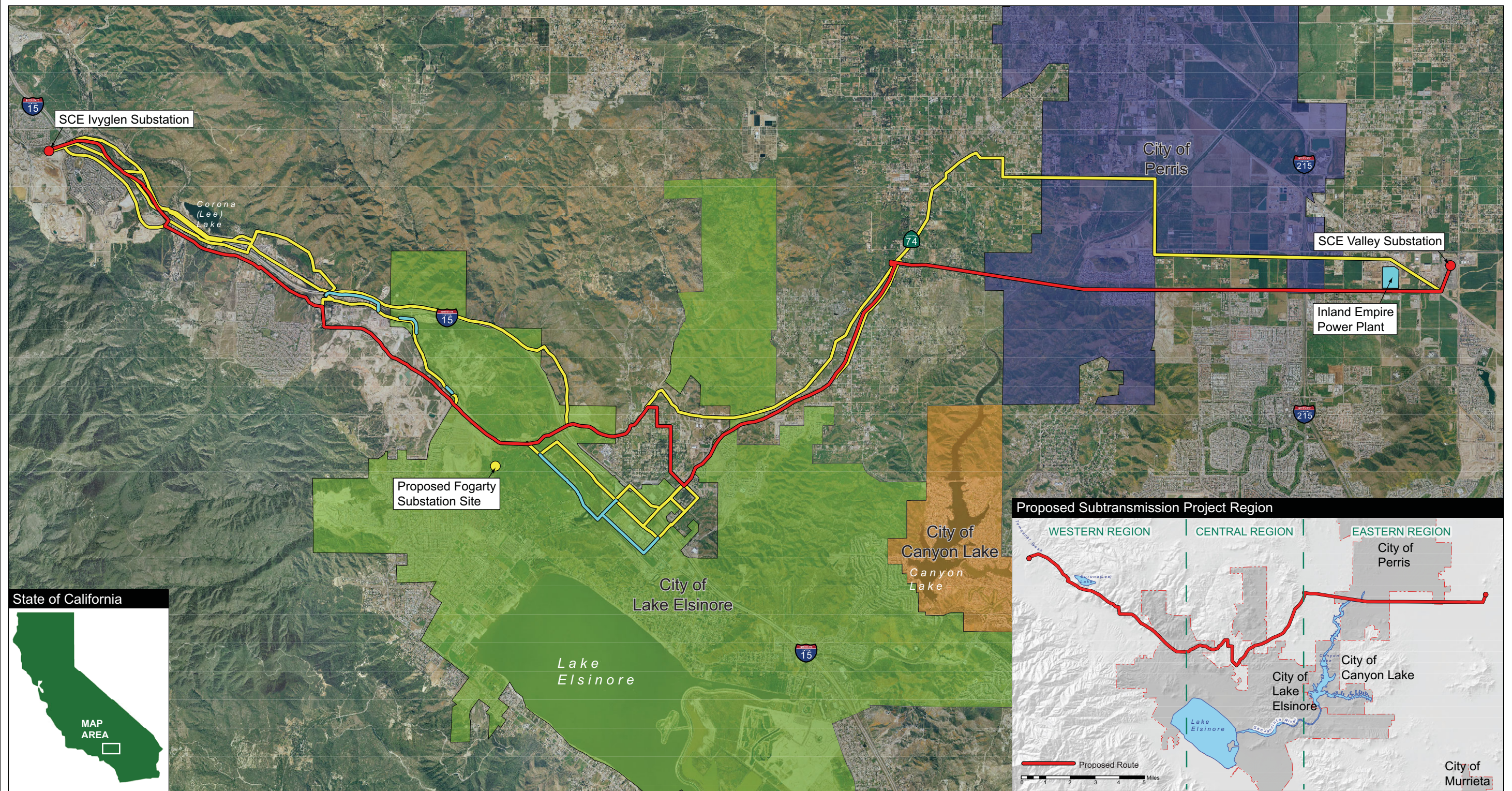
Figure C.2-2 Proposed Subtransmission, Alternative Routes, Power Plant Site, and Proposed New Substation Site
