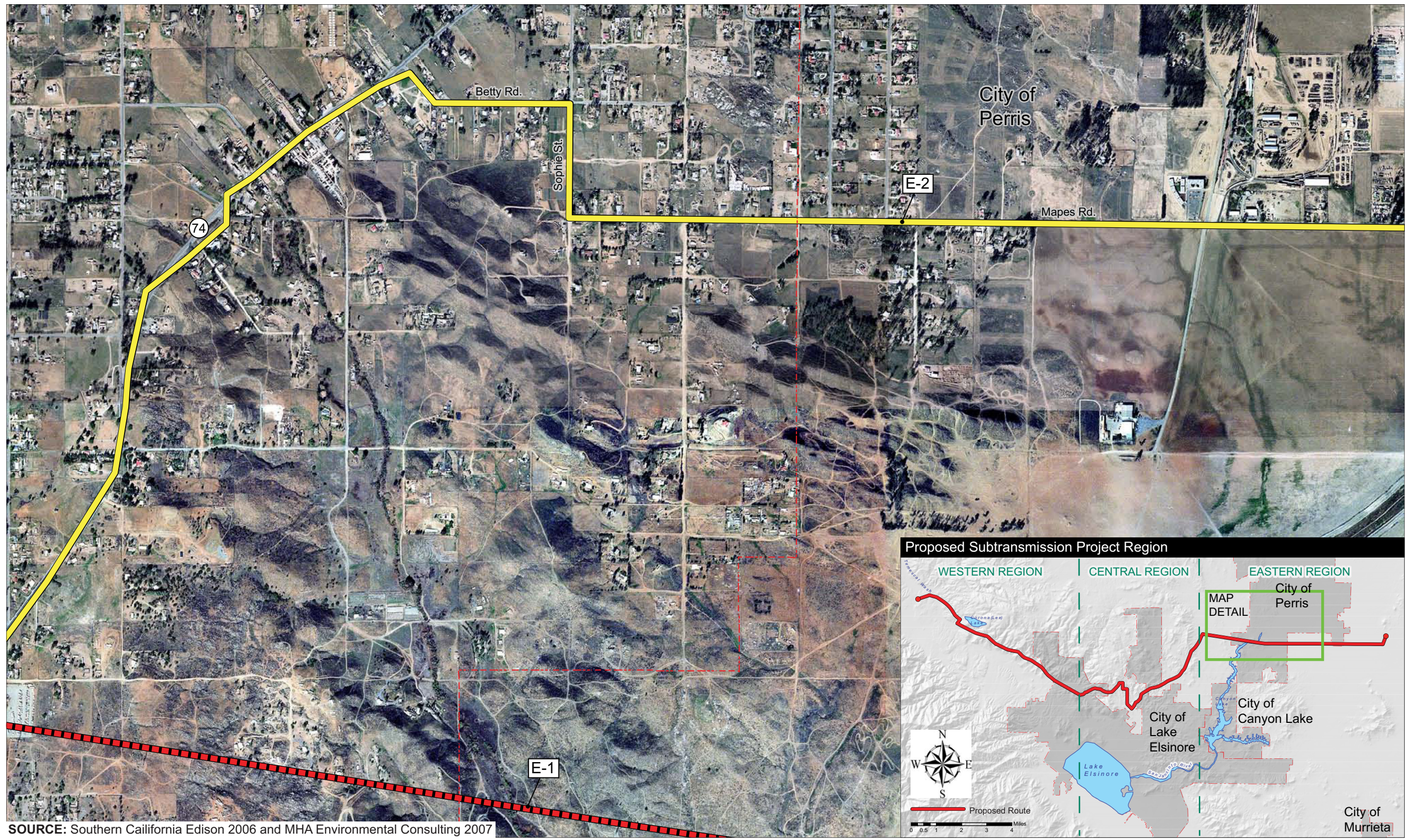
Figure C.2-4 Proposed Subtransmission and Alternative Route Segments
