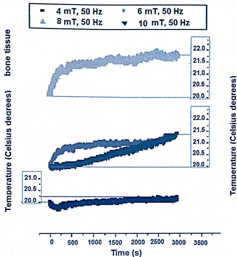
Fig. 8 The temperature recording in bone tissue electromagnetically exposed
