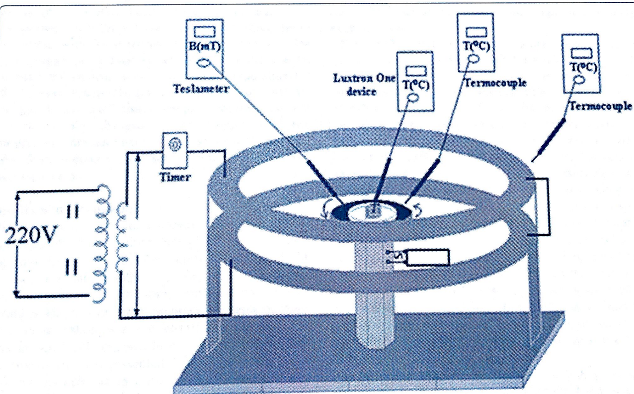
Fig. 1 Experimental set-up; coil system supplied by power transformer connected to industrial electricity grid
