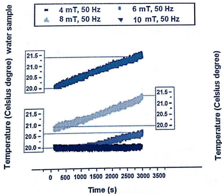
Fig. 9 Deionized water electromagnetically exposed (the volume of 2 \text{ cm}^3 was considered)
