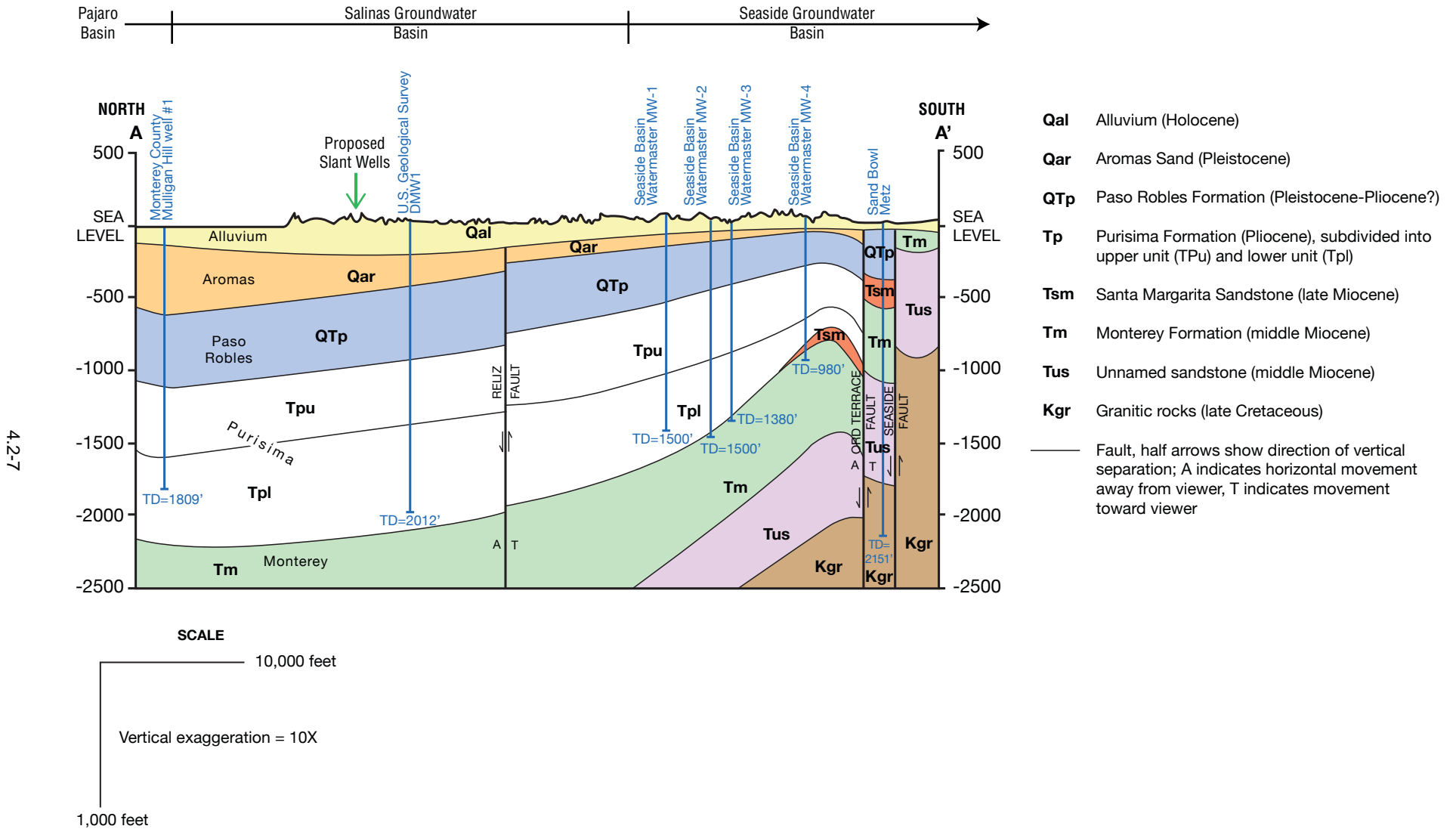
Figure 4.2-2 Generalized Geologic Cross-Section
