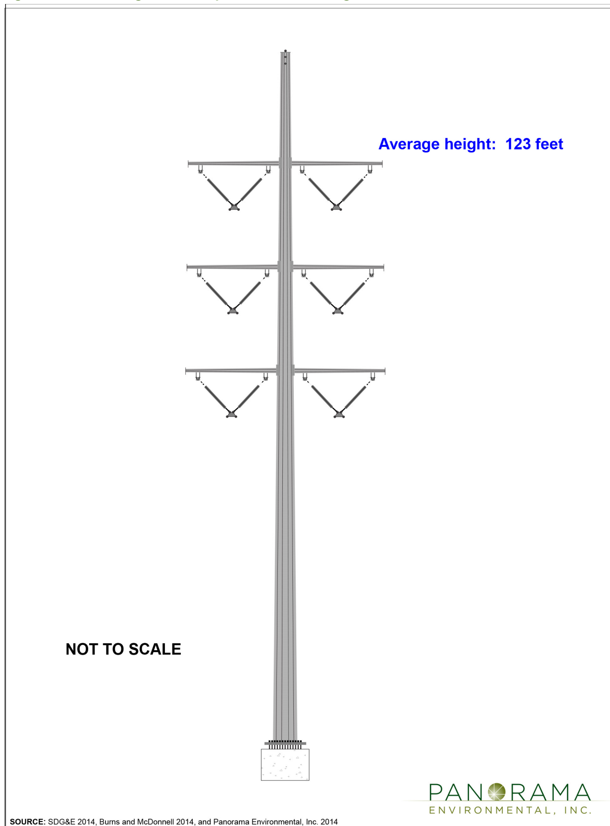
Figure 2.2-10 Diagram of Proposed 230-kV Tangent Double-Circuit TSP
