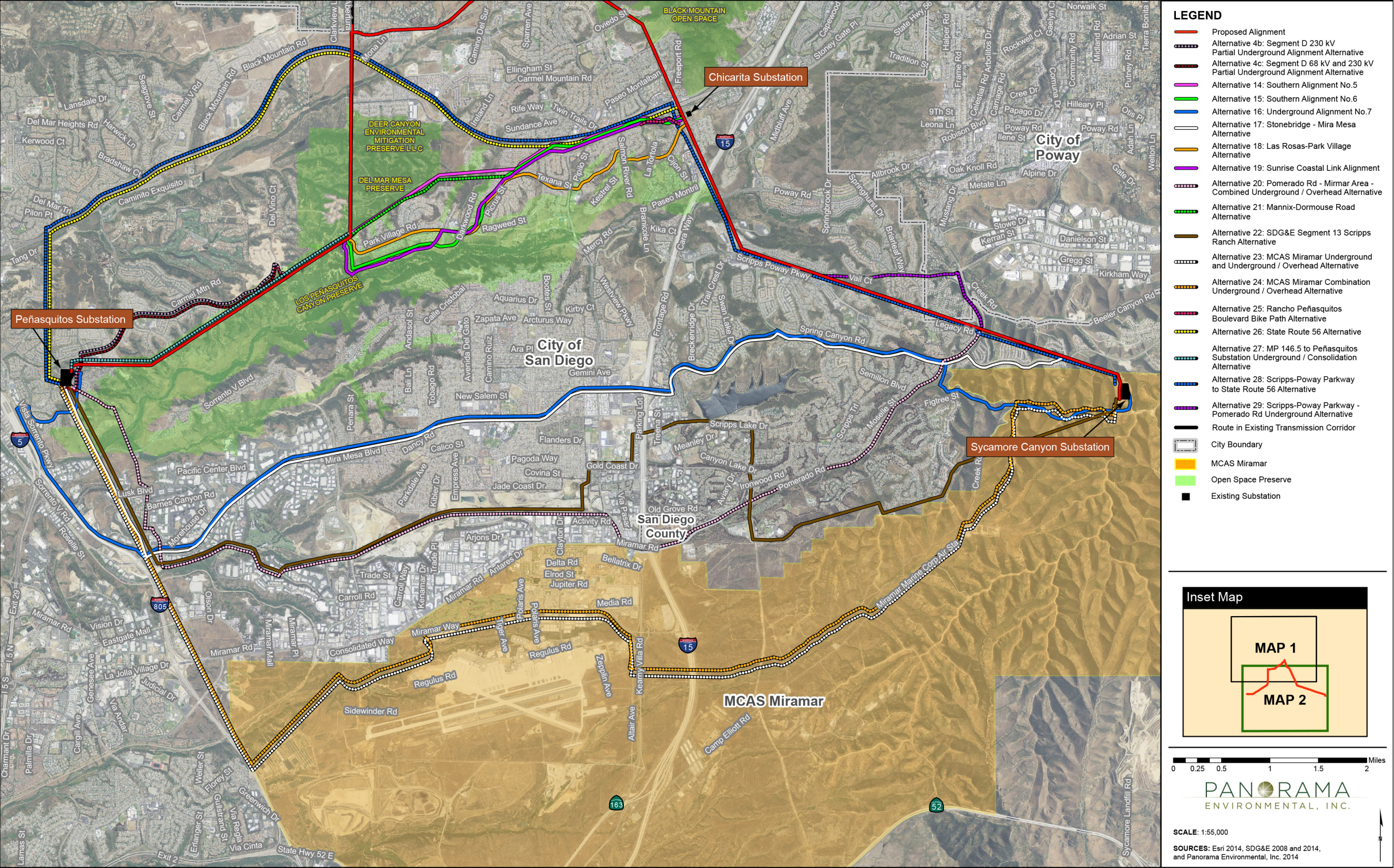
Figure 3.6-4 Eliminated Routing Alternatives (South) (Revised)
