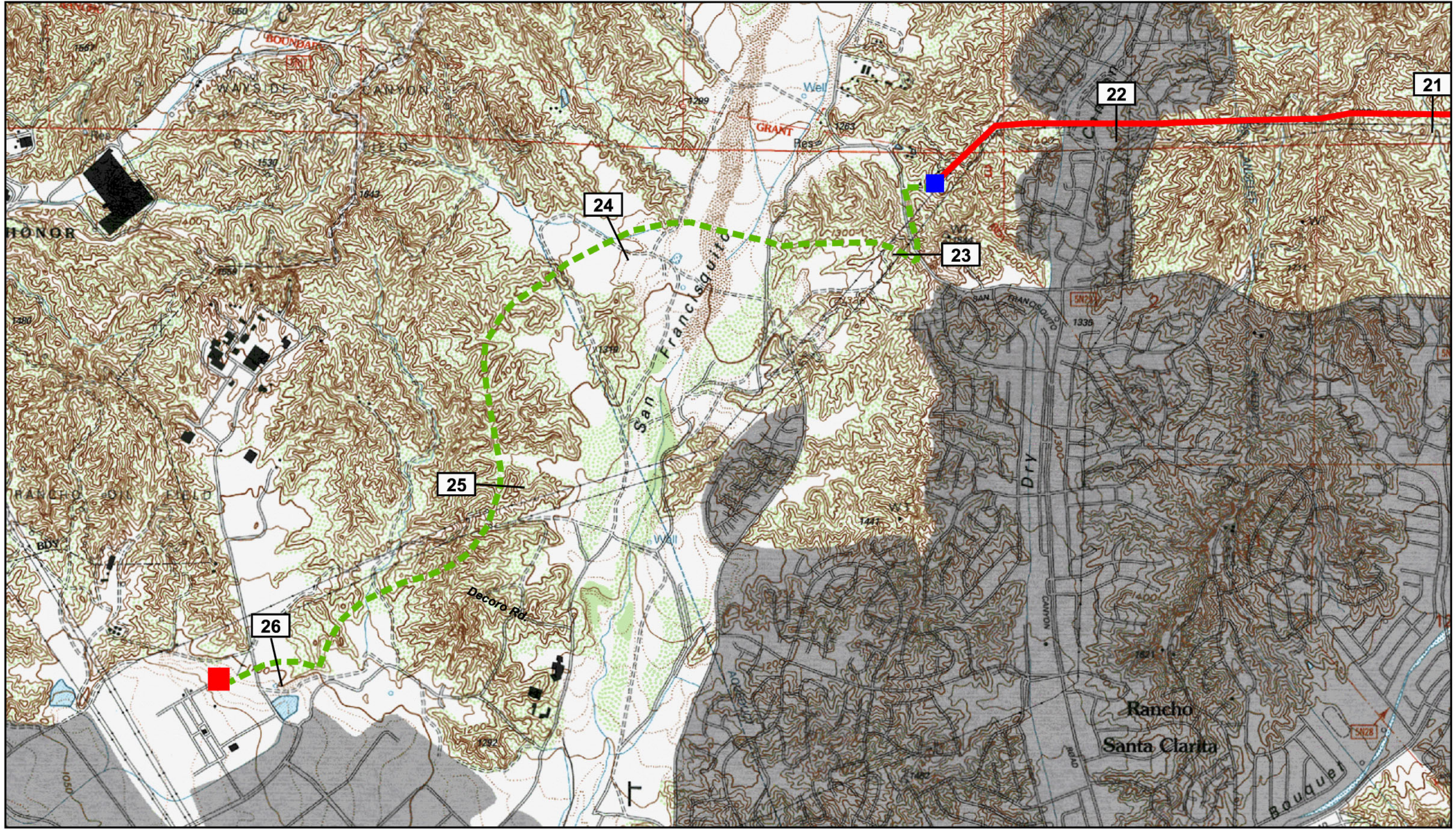
Figure B.4-1b Alternative 1: Underground Segment in Santa Clarita
