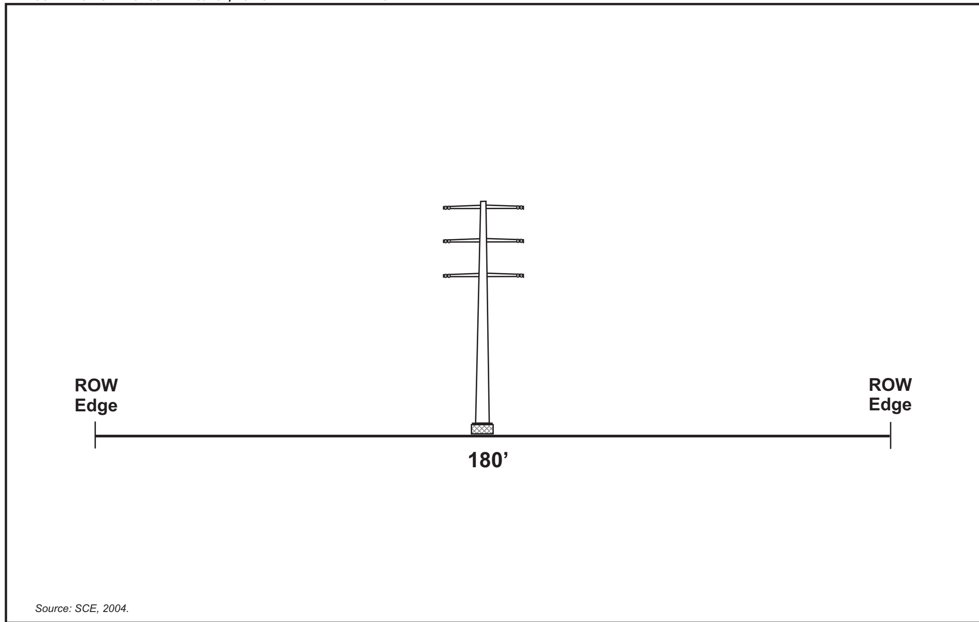
Figure B.2-6 Proposed New ROW Configuration For Proposed Project Mile 0 to Mile 0.1
