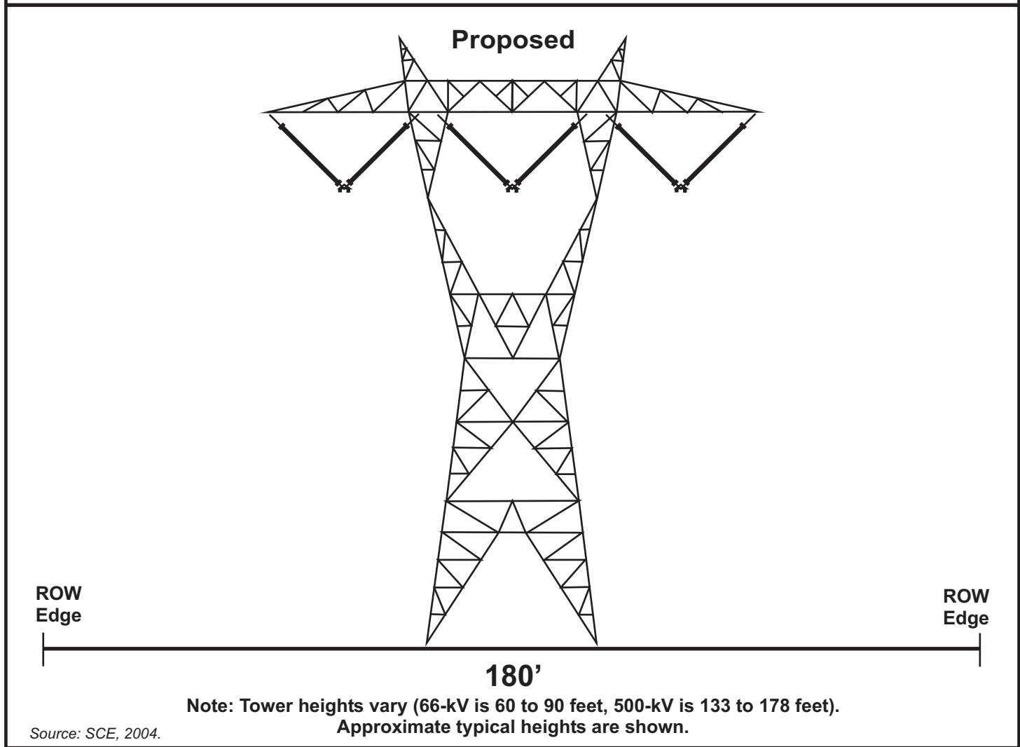
Figure B.2-8 Existing and Proposed ROW Configurations For Proposed Project Mile 1.1 to Mile 5.7 PREPARED BY Aspen Environmental Group
