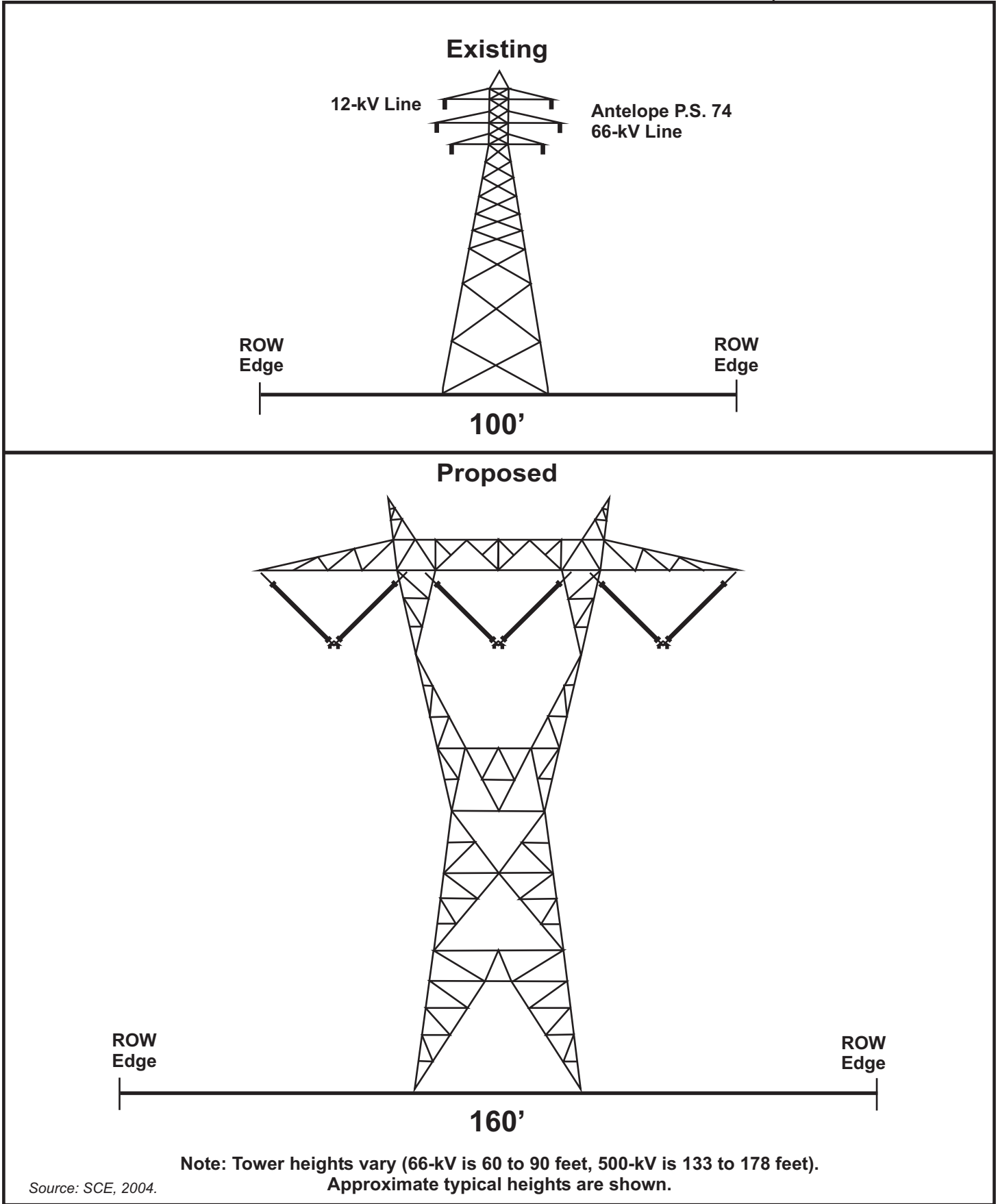
Figure B.2-9 Existing and Proposed ROW Configurations For Proposed Project Mile 5.7 to Mile 18.6
