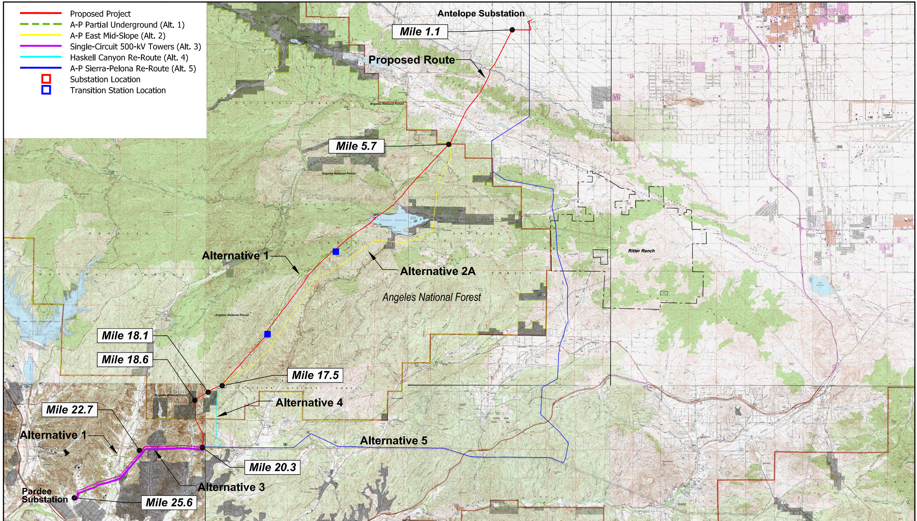
Figure ES-2 Antelope Pardee 500-kV Proposed and Alternative Routes
