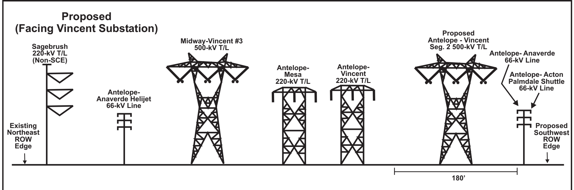
Figure B.2-15 Existing and Proposed ROW Configurations for Mile S2-1.9 to Mile S2-4.4
