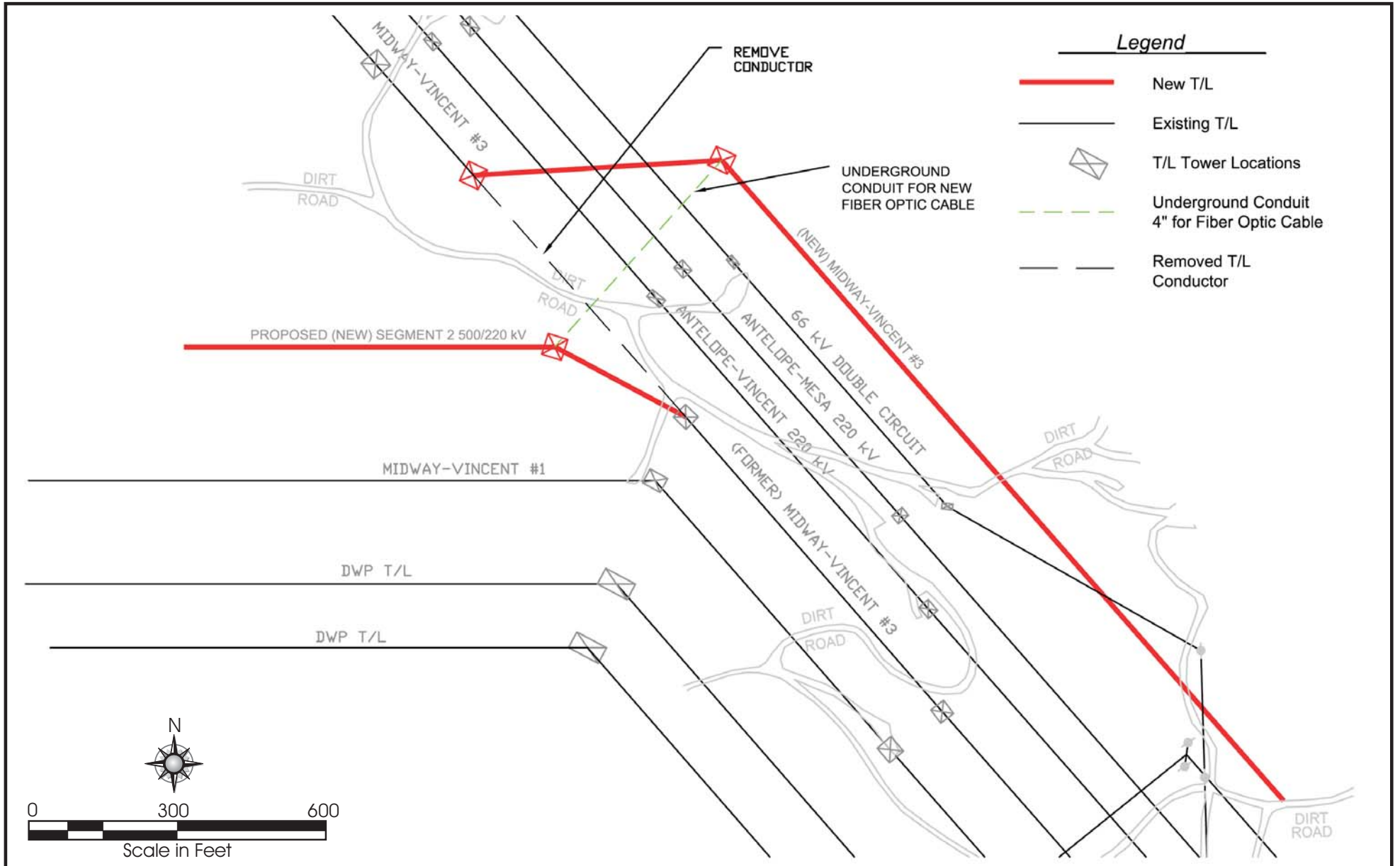
Figure B.2-20 Line Diagram of the Connection to Midway-Vincent No. 3 at Mile S2-14.8
