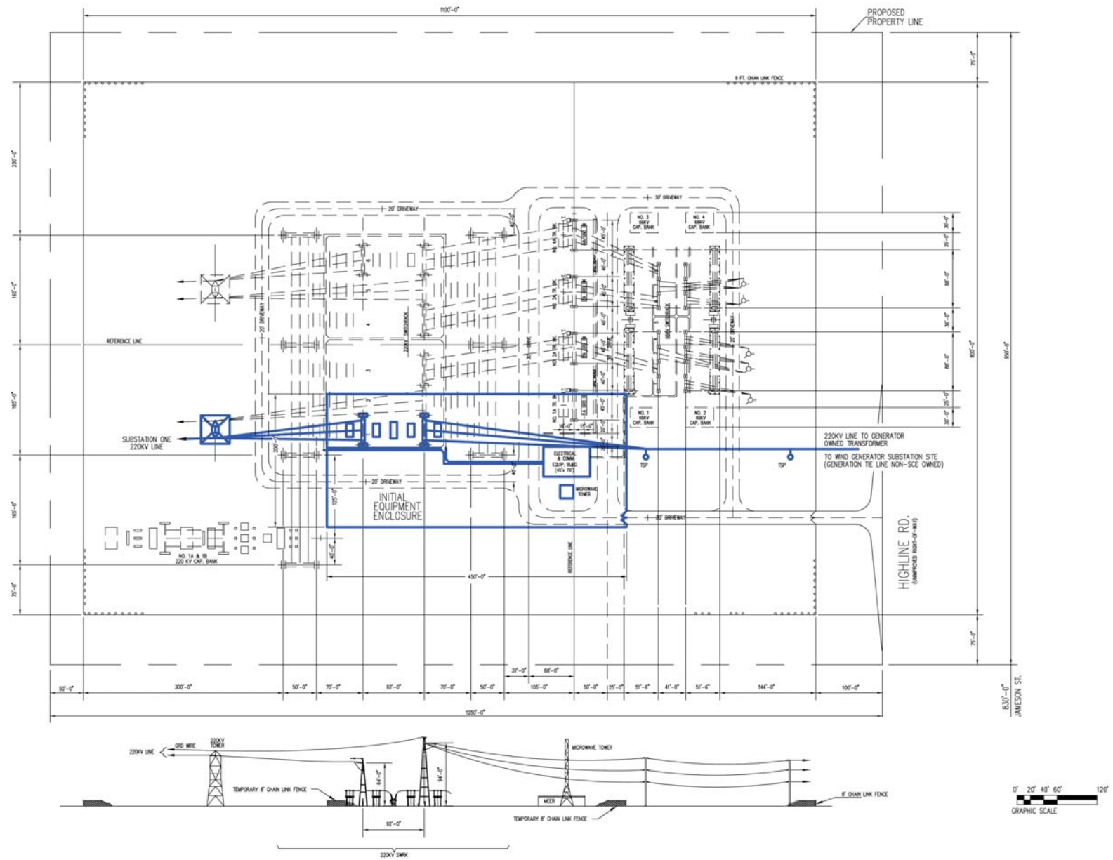
Figure B.2-26 Proposed Substation Two Plot Plan
