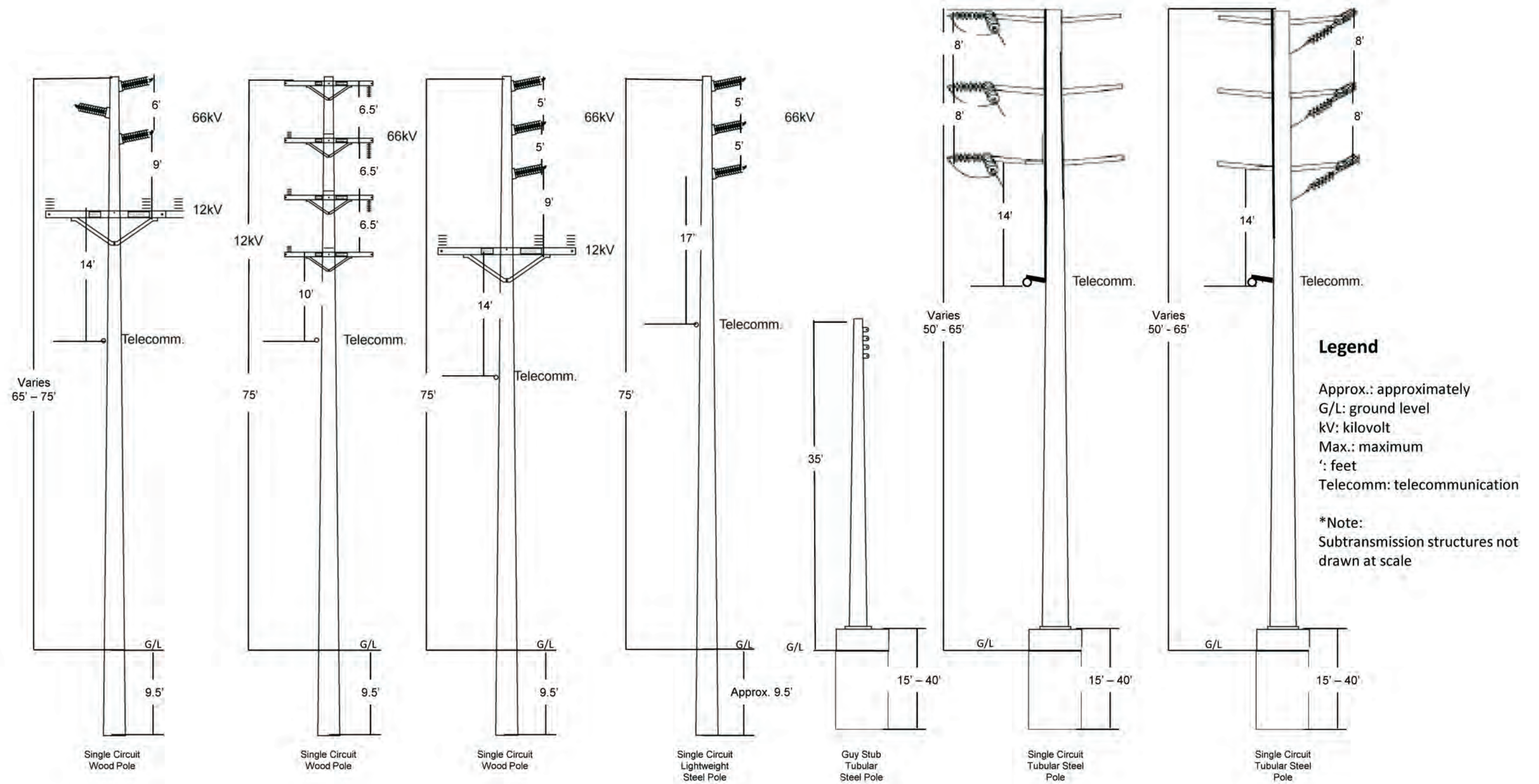
Figure 4-4 Subtransmission Structures
