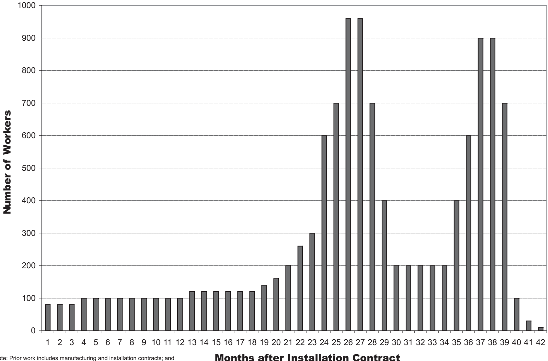
DCPP Steam Generator Replacement Figure B-16
