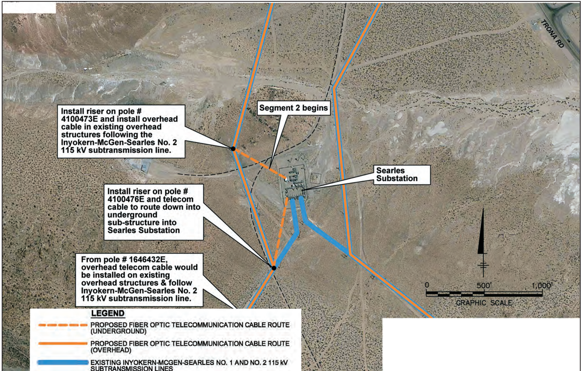
Figure B.1-13 (Revised) Proposed Fiber Optic Telecommunication Cable Route - Segments 1 and 2
