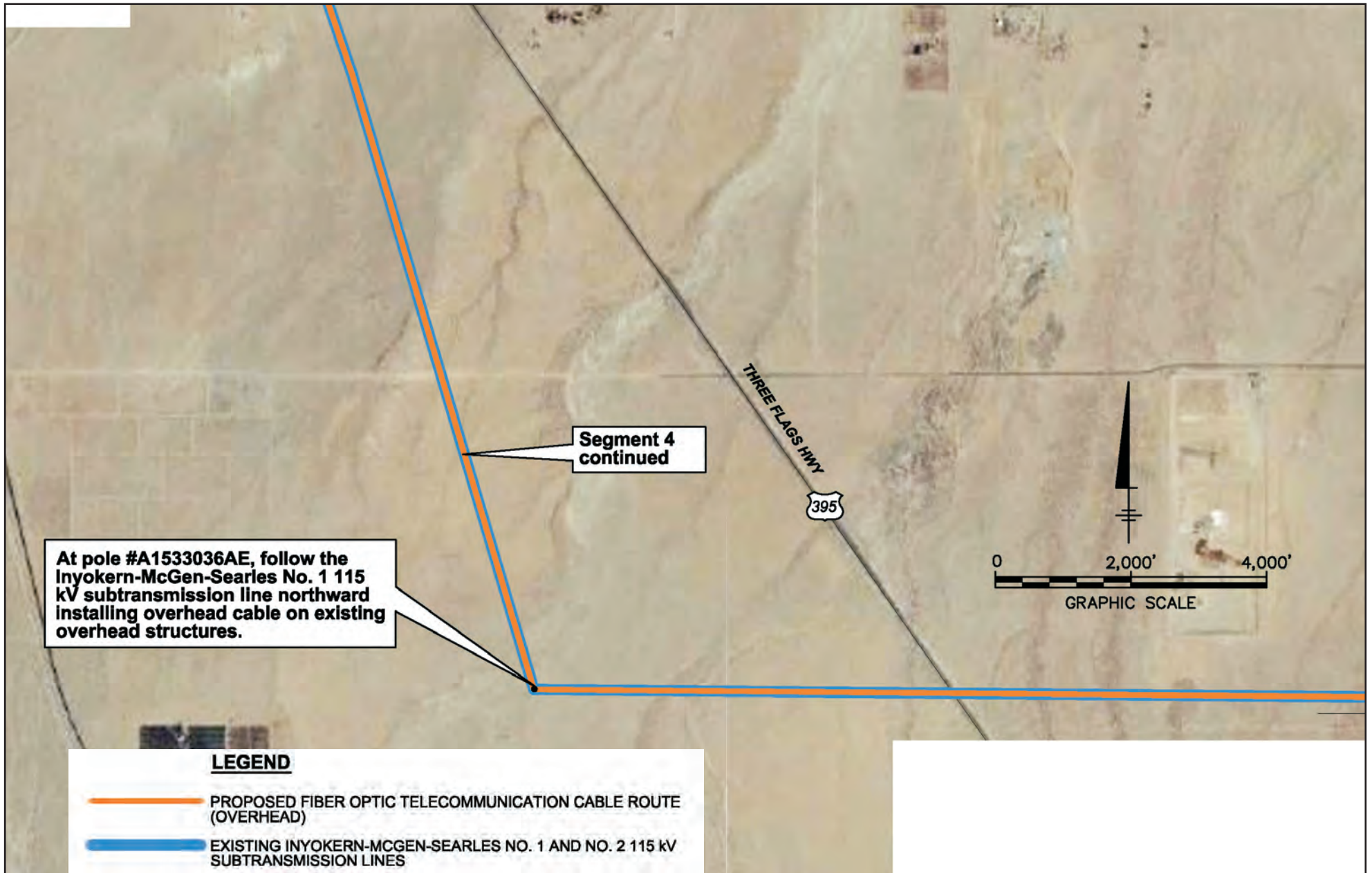
Figure B.1-16 Proposed Fiber Optic Telecommunication Cable Route - Segment 4 (Continued Southern Part)
