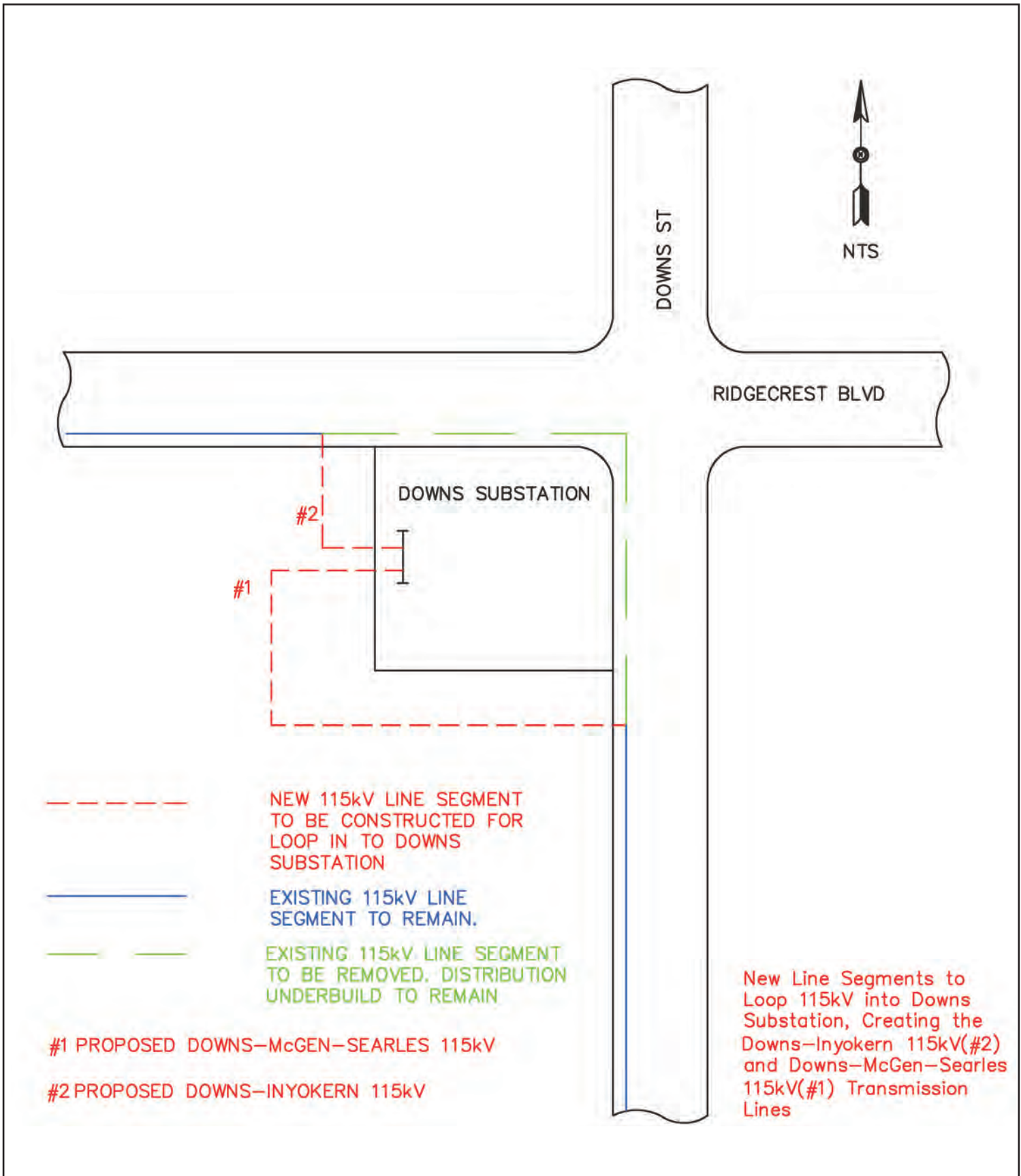
Figure B.1-2 New Downs 115/12 kV Substation 115 kV Looped Configuration
