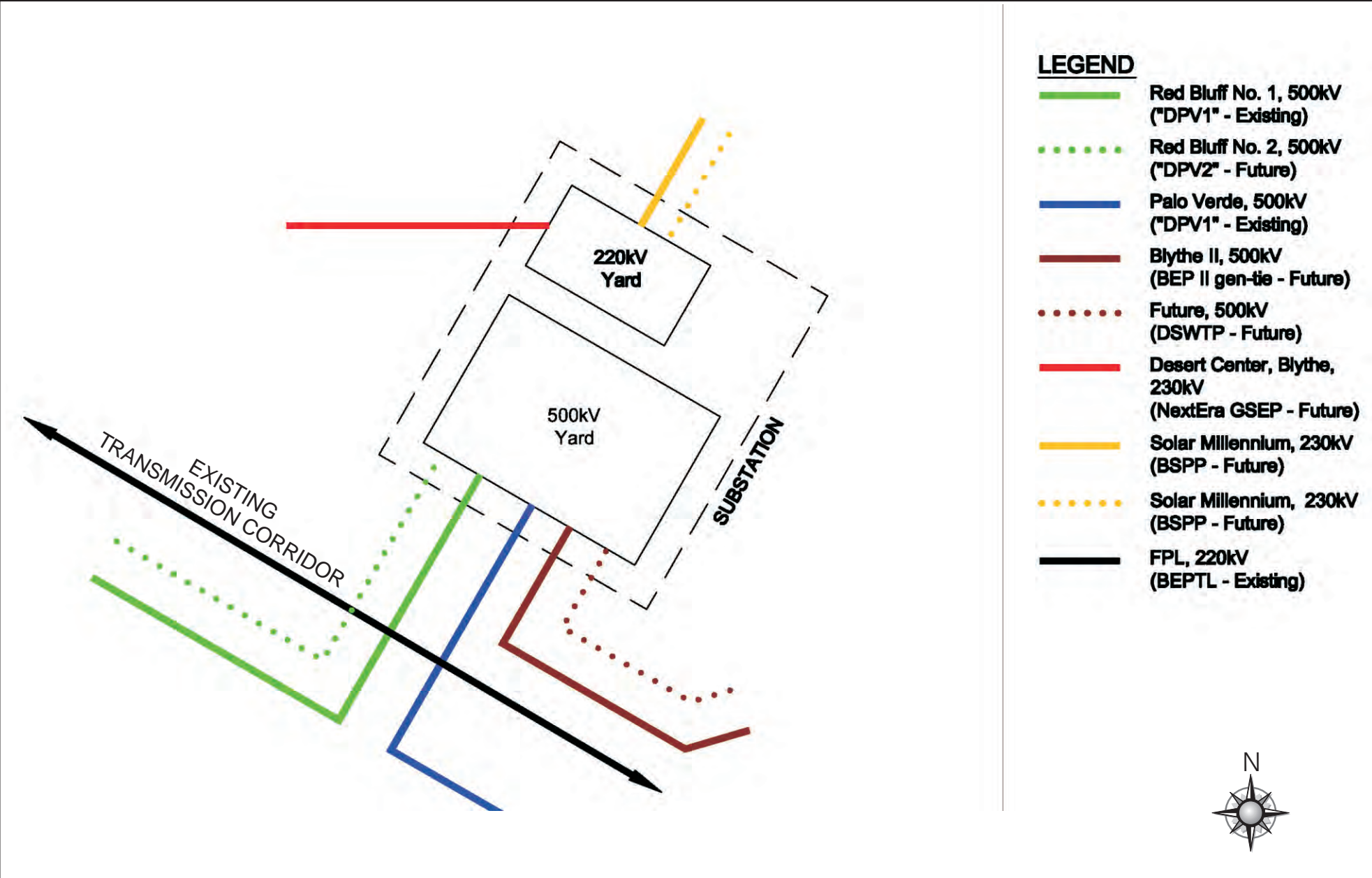
Figure Ap.1-3B Avoidance Alternatives Substation Configuration (Perpendicular Orientation)
