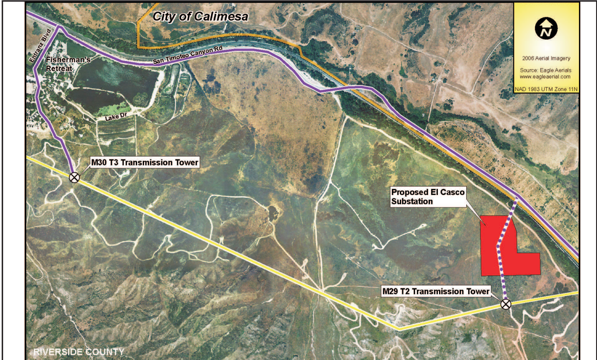
Figure B-14 Fiber Optic Cables in the Vicinity of El Casco Substation
