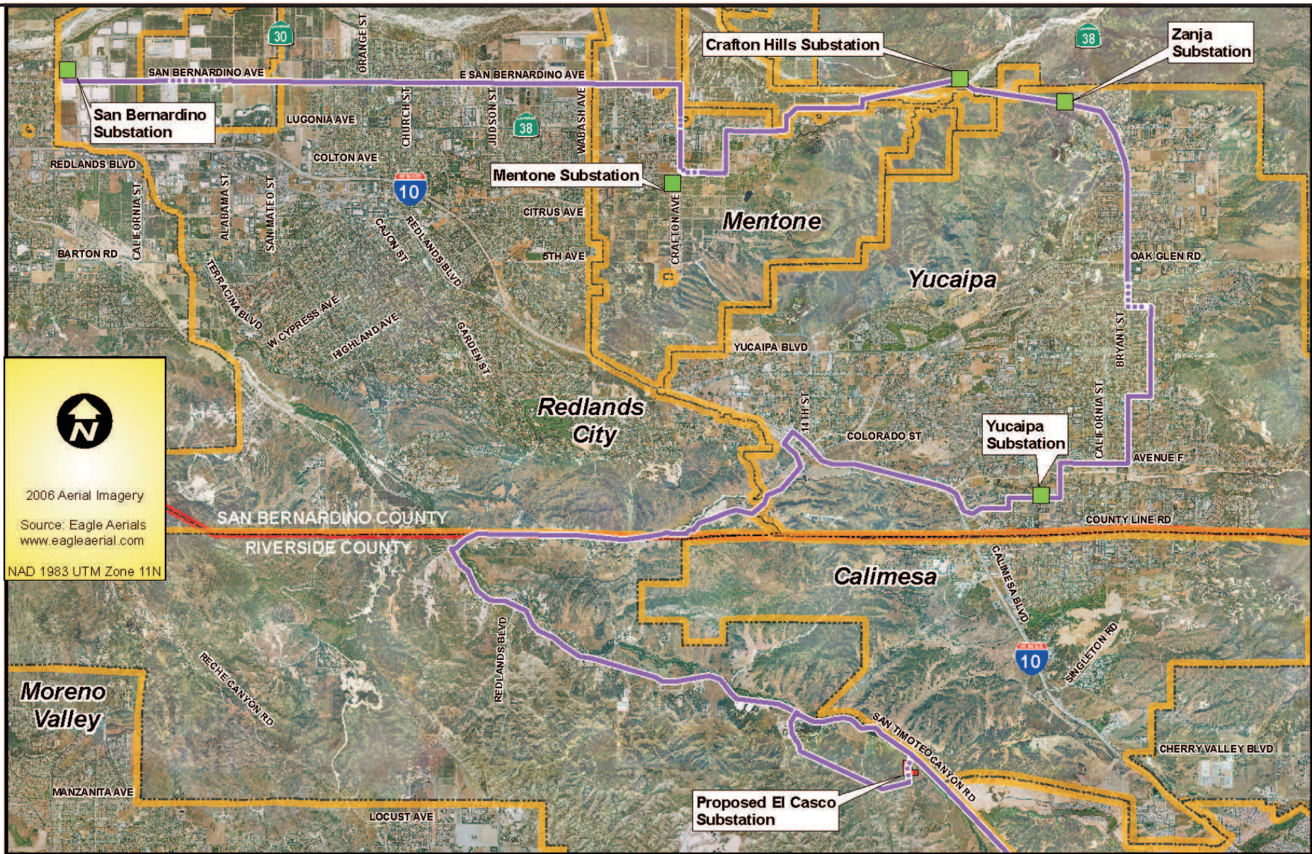
Figure B-12 El Casco-San Bernardino Fiber Optic Cable Route
