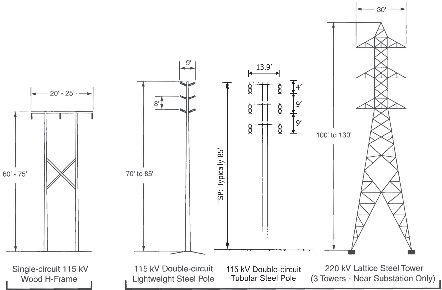
Figure B-5 Typical Structure Designs
